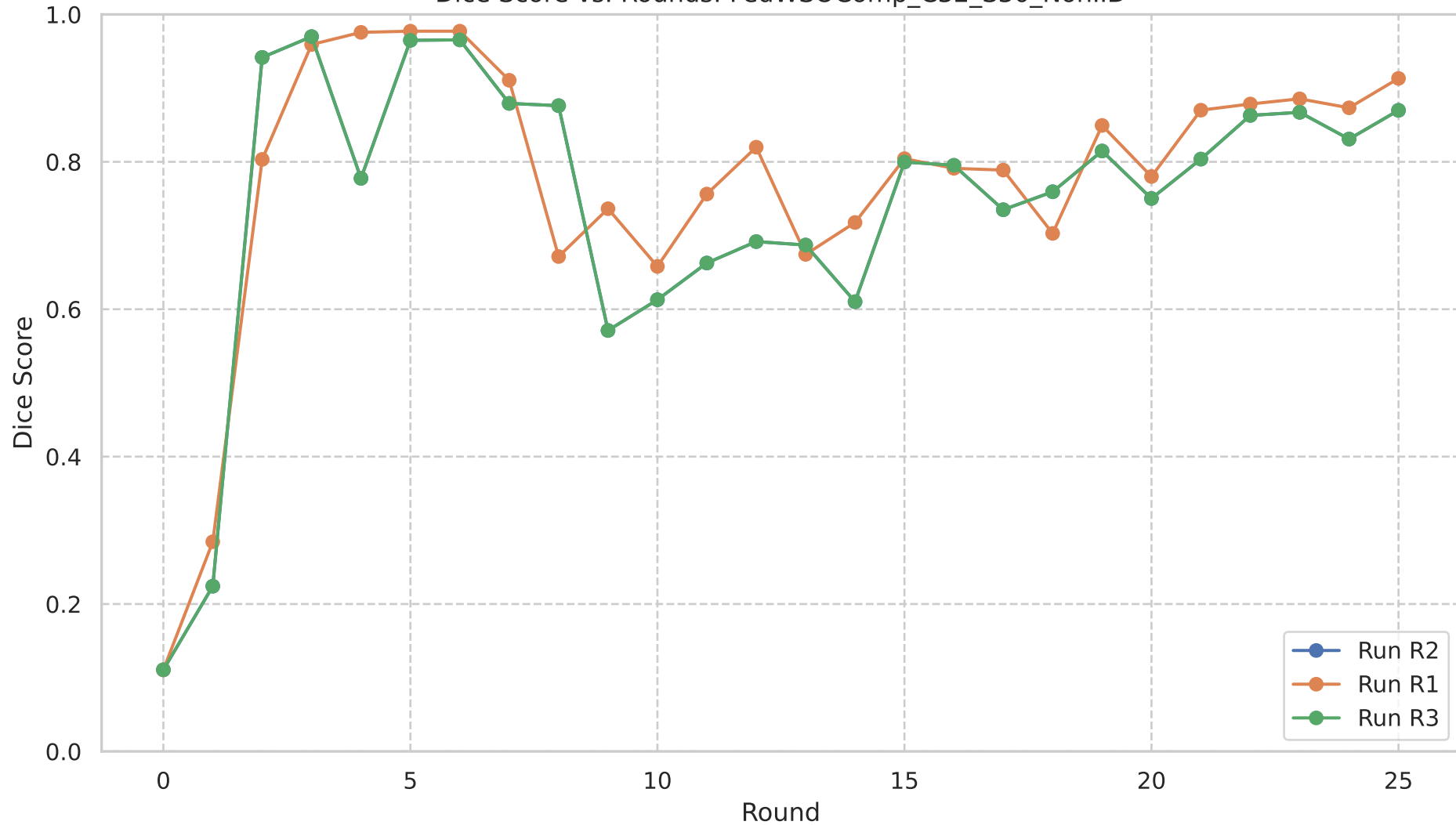
Dice Score vs. Rounds: FedWSOComp_C32_S30_NonIID
