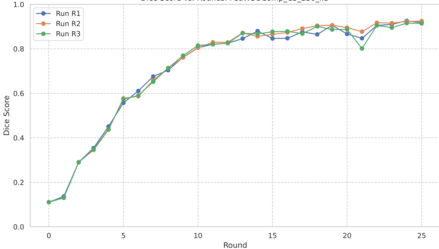
Dice Score vs. Rounds: FedWSOComp_C3_S30_IID
