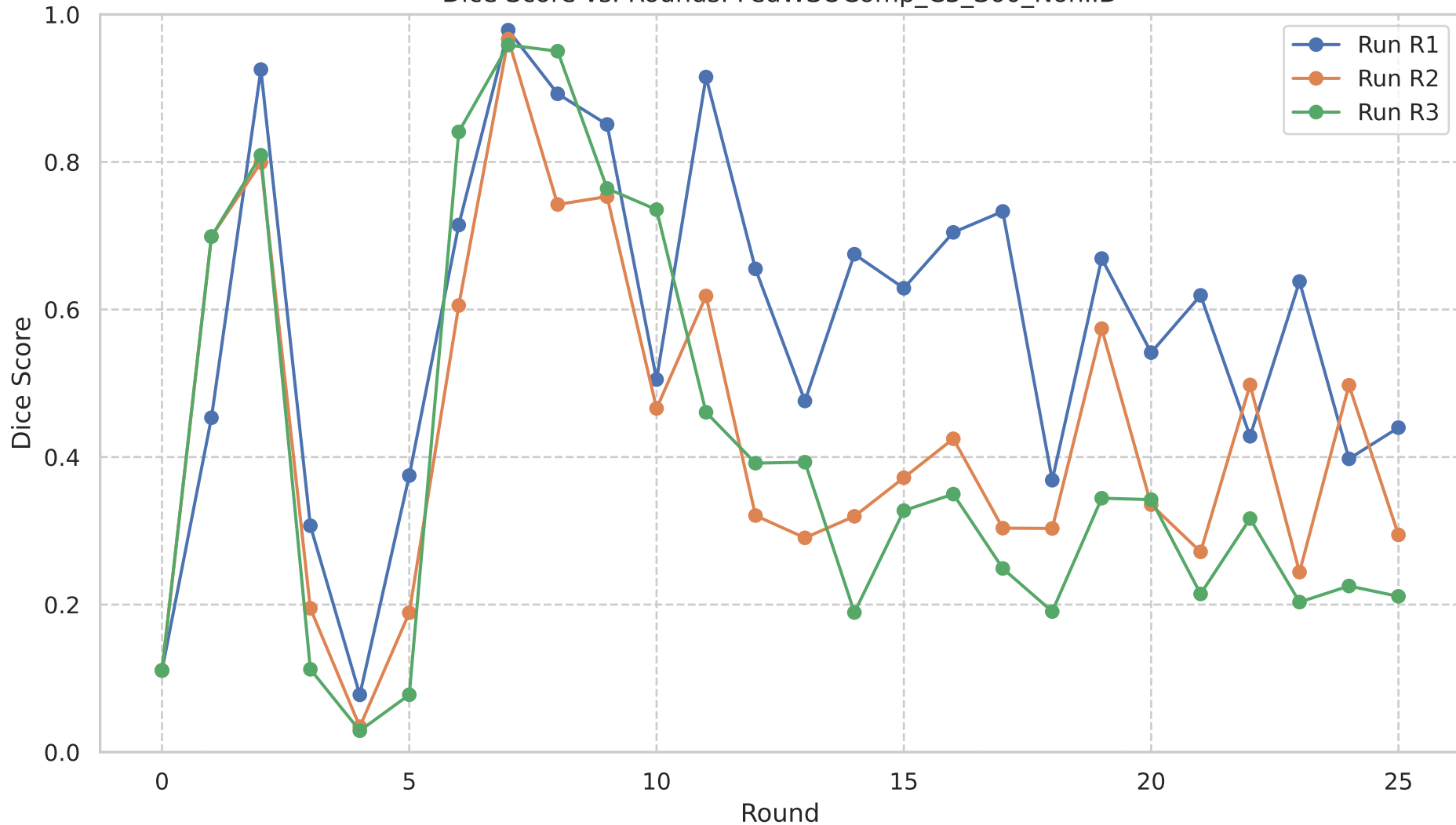
Dice Score vs. Rounds: FedWSOComp_C3_S60_NonIID
