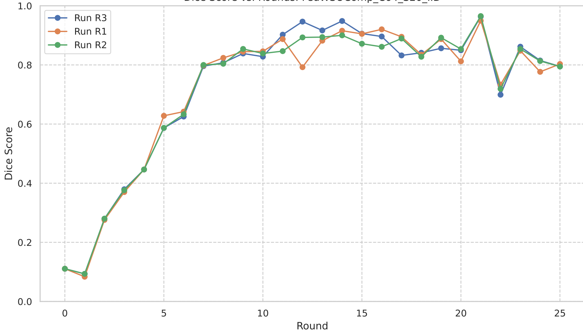
Dice Score vs. Rounds: FedWSOComp_C64_S20_IID
