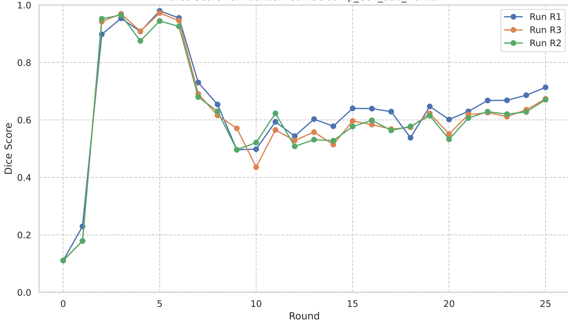
Dice Score vs. Rounds: FedWSOComp_C64_S20_NonIID
