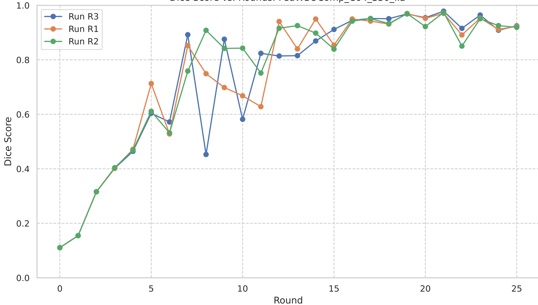
Dice Score vs. Rounds: FedWSOComp_C64_S30_IID
