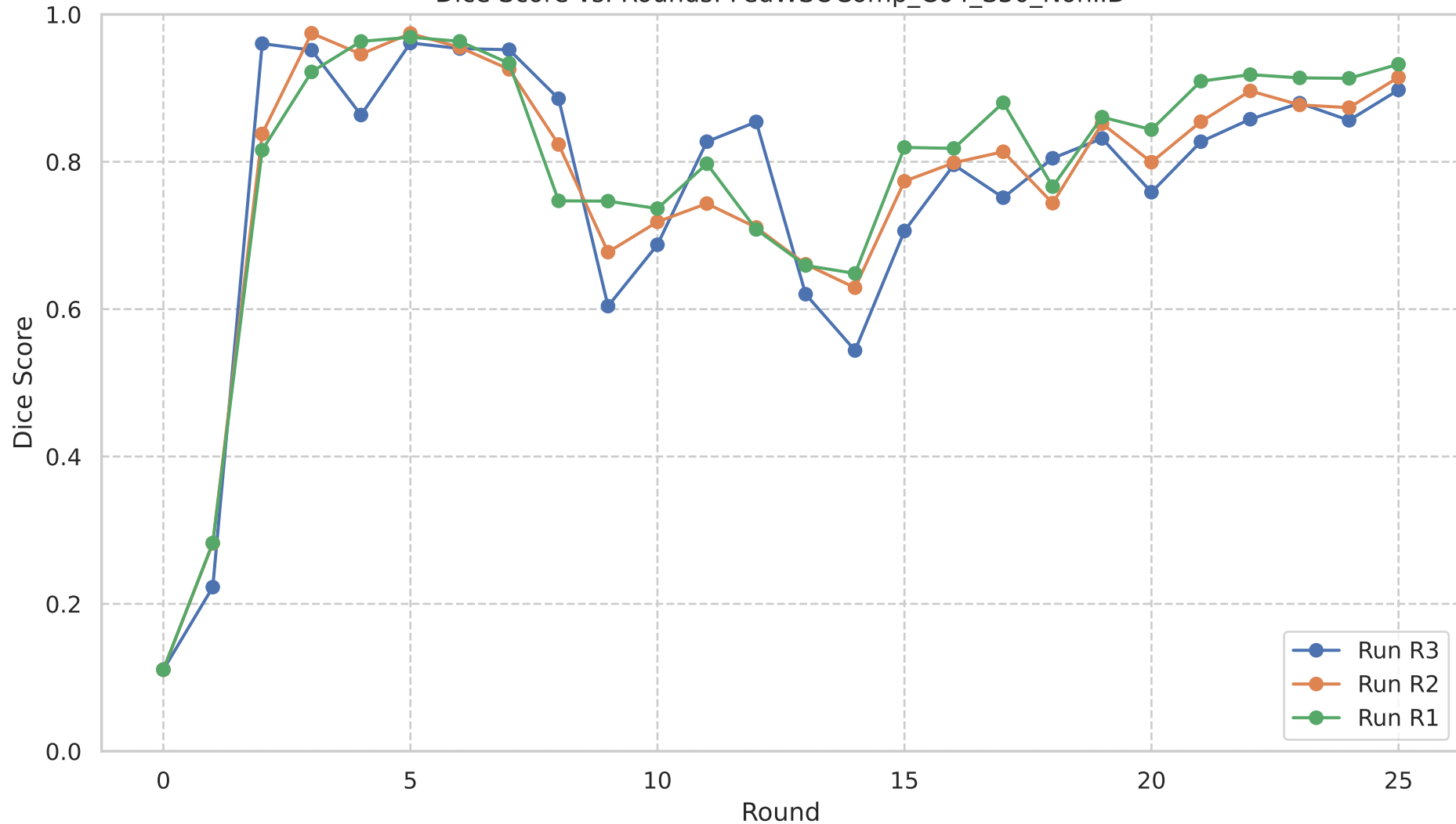
Dice Score vs. Rounds: FedWSOComp_C64_S30_NonIID
