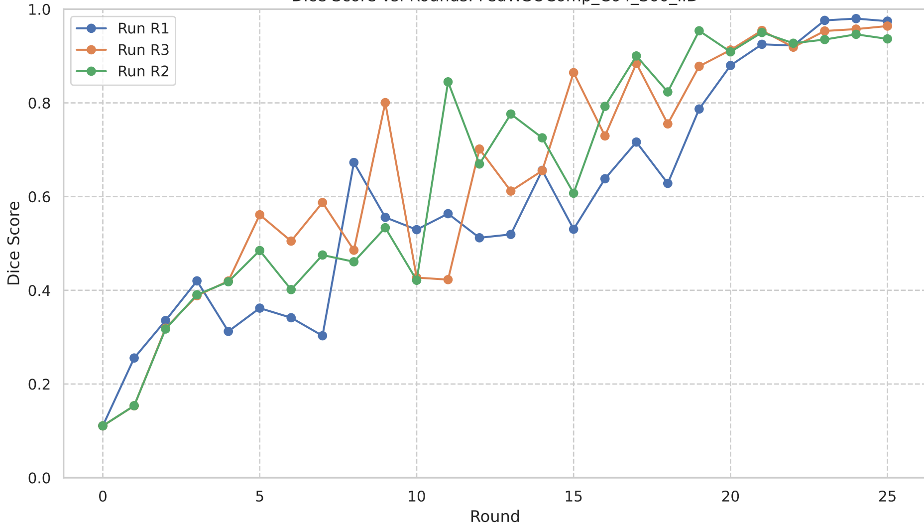
Dice Score vs. Rounds: FedWSOComp_C64_S60_IID
