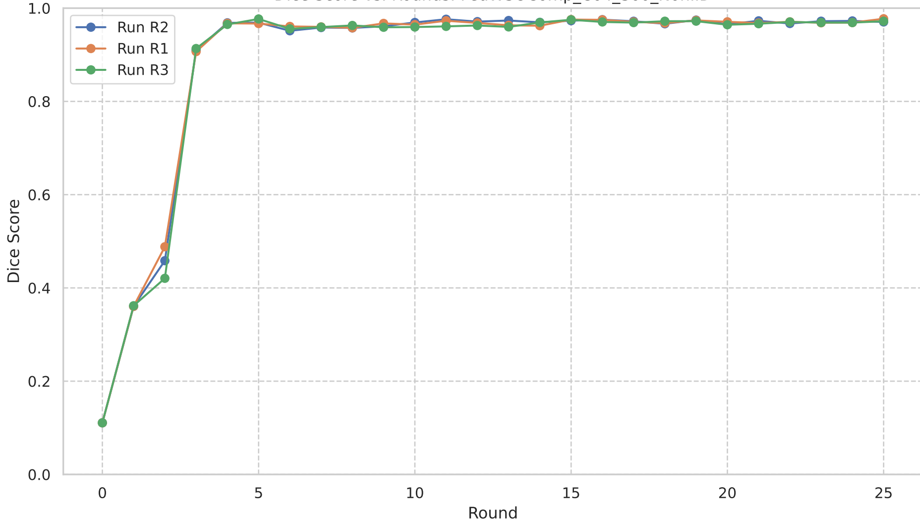
Dice Score vs. Rounds: FedWSOComp_C64_S60_NonIID
