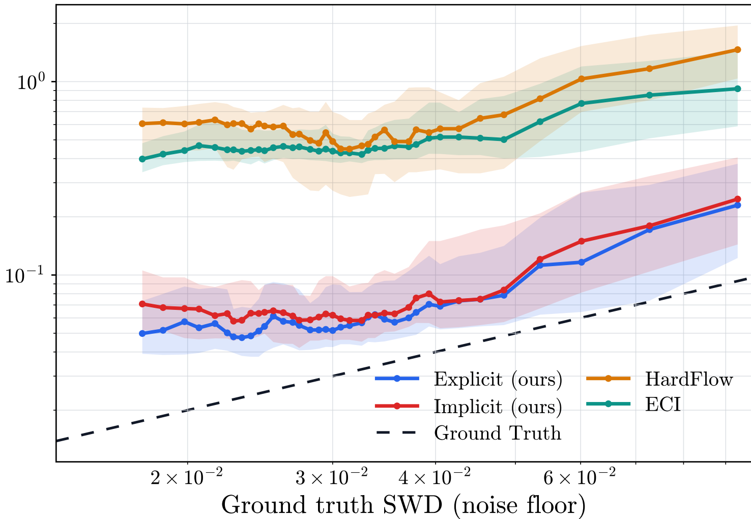
Sliced Wasserstein Distance
