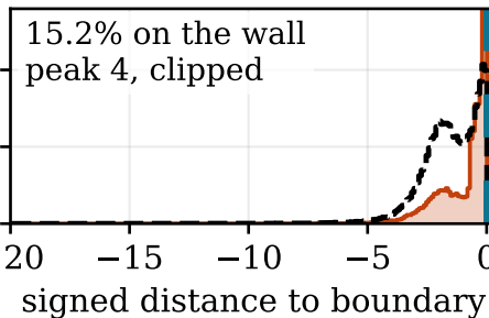
HardFlow
