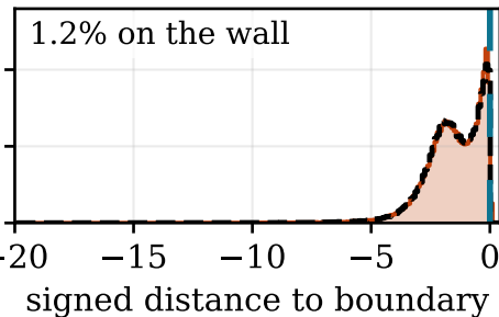
Constraint Amortization
