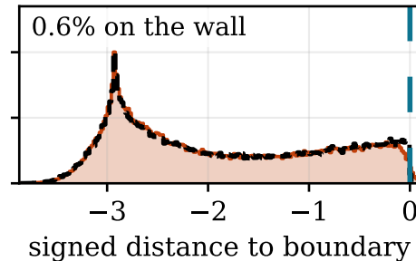
Constraint Amortization
