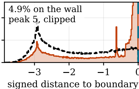
HardFlow
