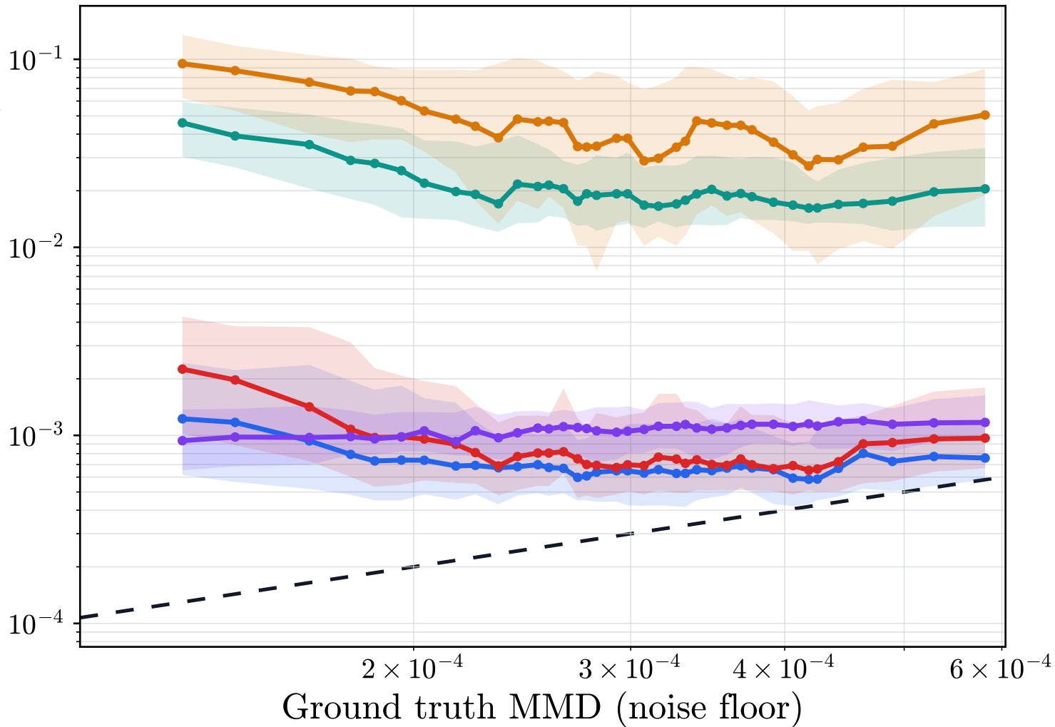
Maximum Mean Discrepancy
