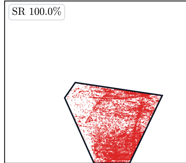
HardFlow
