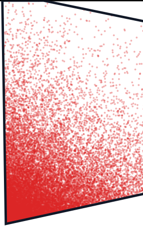
Ground Truth
