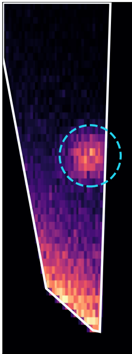
Exact conditional
