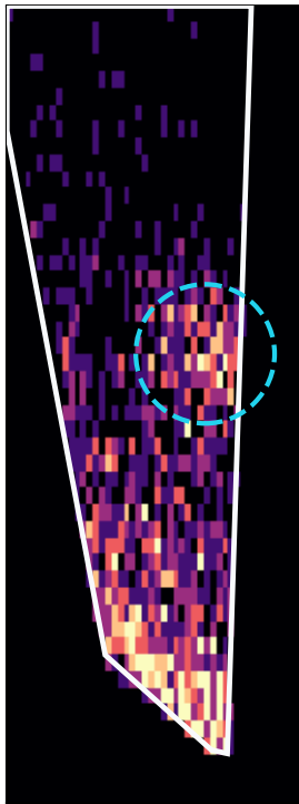
Rejection filtering
