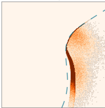
HardFlow (inference guidance)
