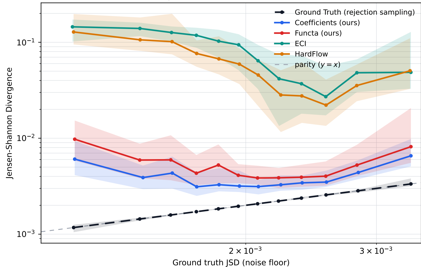
JSD against the achievable noise floor
