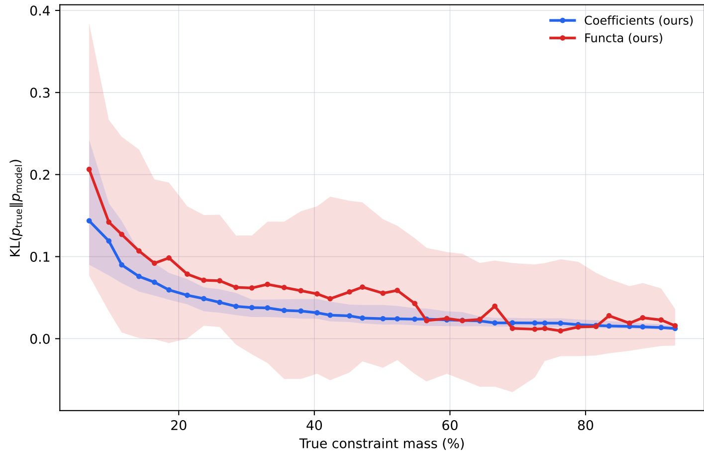
KLD vs constraint mass (exact likelihood)
