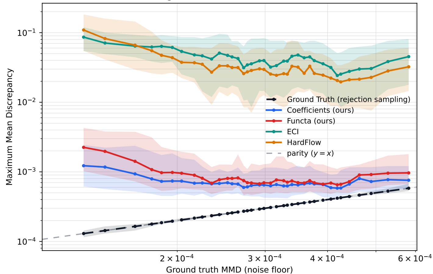
MMD against the achievable noise floor
