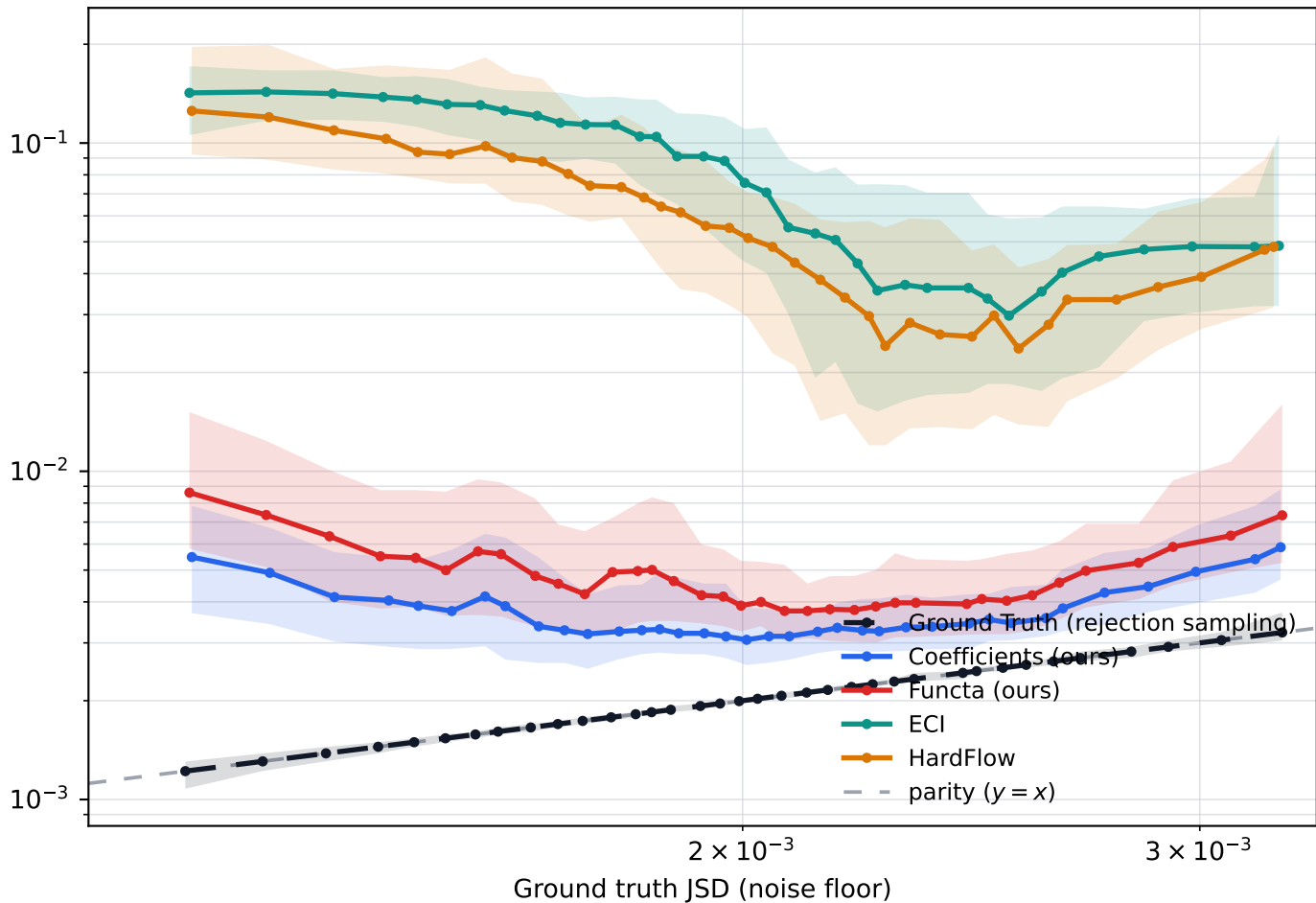
Jensen-Shannon Divergence
