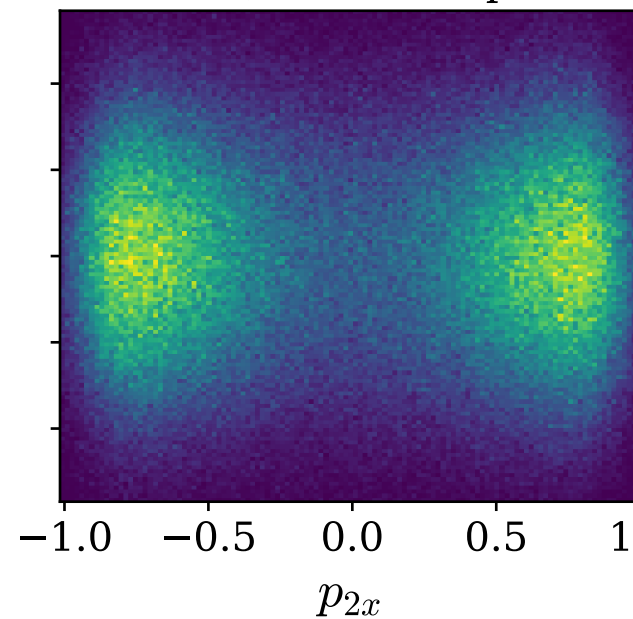
IS, learned p
