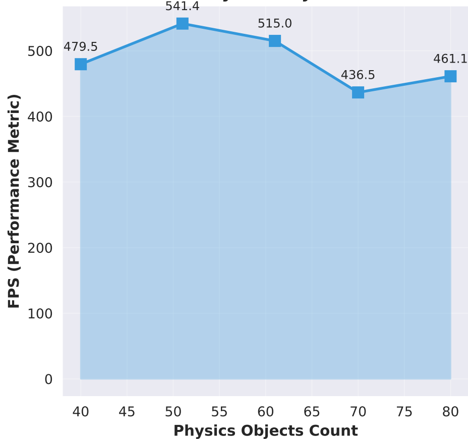
Effect of Physics Objects on FPS
