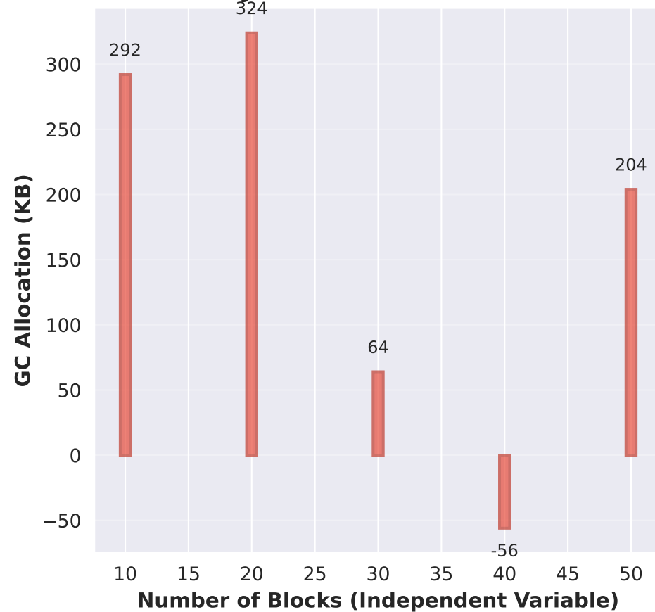
Memory Allocation vs Block Count
