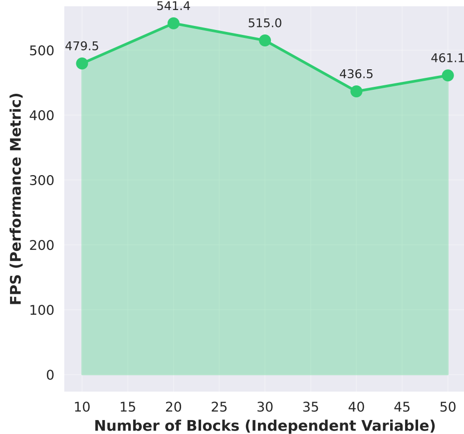
Effect of Block Count on FPS
