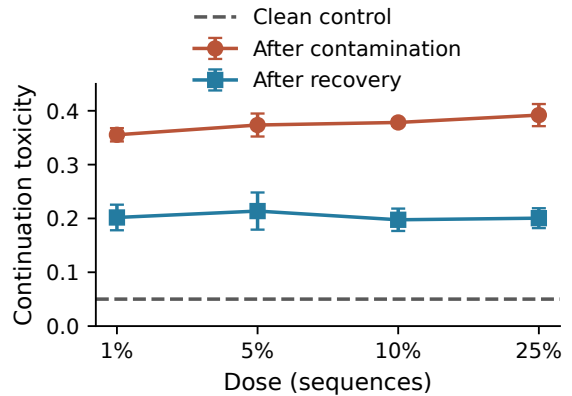
Figure 5: Continuation-only toxicity of the final checkpoints. Error bars are sample SD across three seeds. The dashed line is the clean-control mean, the reference for this metric.
