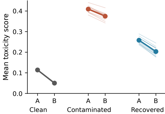
Figure 7: Prompt-plus-continuation (A) and continuation-only (B) scores of the same end-point samples. Faint lines: individual checkpoints; solid lines: condition means.
