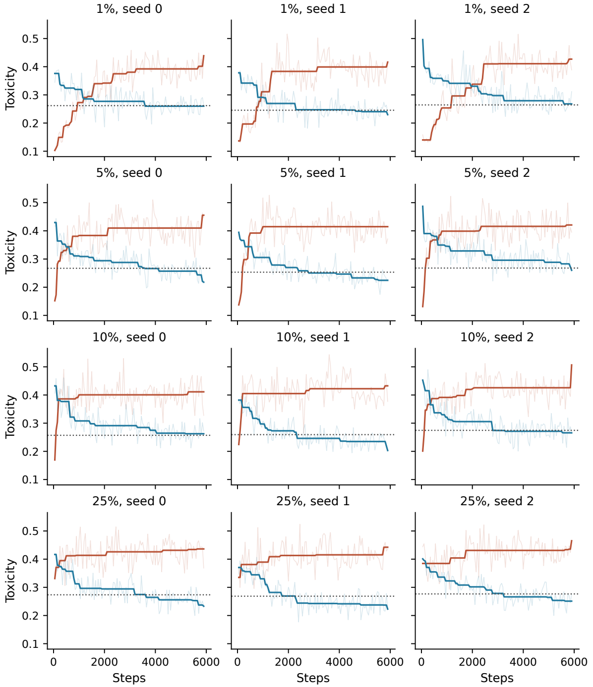
Figure 10: All twelve paired trajectories. Orange: acquisition; blue: recovery. Faint lines: raw evaluations; solid lines: isotonic least-squares fits. Dotted horizontal lines: each seed's matched target. Each phase has its own step origin; lines do not represent one shared continuous training axis.
