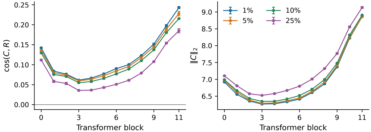
Figure 6: Per-block endpoint geometry. Left: contamination–recovery cosine. Right: contamination displacement norm. Error bars are sample SD across three seeds. Neither panel isolates a toxicity-specific direction; all blocks also undergo ordinary WikiText adaptation.
