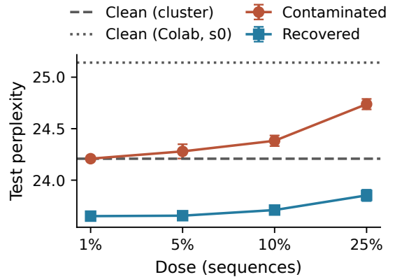
Figure 8: WikiText-103 test perplexity of the final checkpoints. Error bars are sample SD across three seeds. Dashed: mean of the cluster-trained clean seeds; dotted: the Colab-trained clean seed 0. Pretrained GPT-2 scores 51.19.
