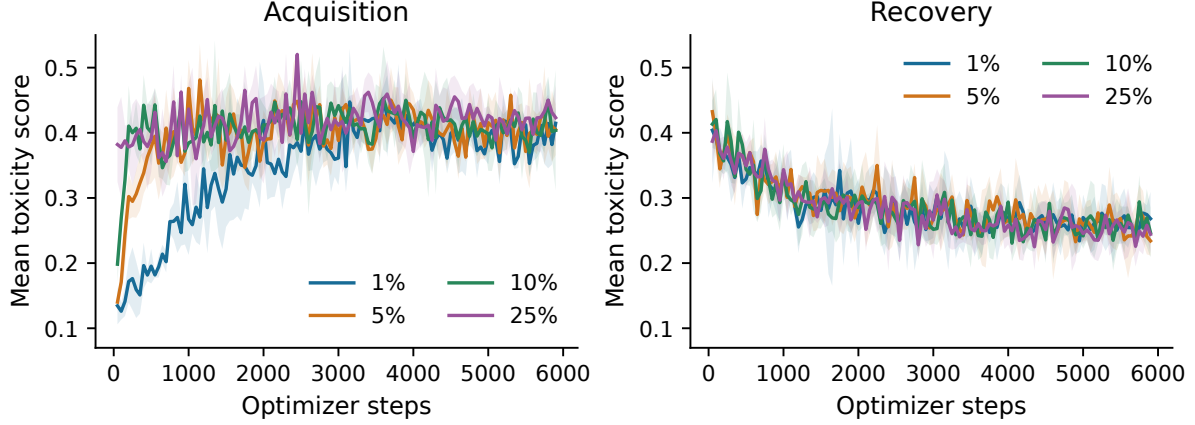
Figure 3: Observed acquisition and recovery trajectories. Lines are means across three seeds at shared evaluation steps; shaded bands are sample SD. These are prompt-plus-continuation scores. Smoothing is applied to individual runs for crossing analysis, not to the plotted dose means.
