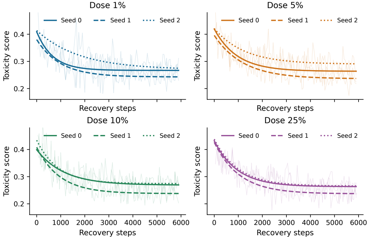
Figure 9: Individual recovery fits anchored to the contamination endpoint estimates. Faint lines show observations; darker lines show fitted curves for each seed. Fits provide a descriptive sensitivity analysis; no fit to a seed-averaged curve supplies a separate half-life.
