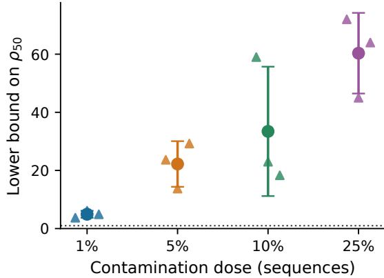
Figure 3: Matched-threshold asymmetry. Triangles show each seed’s lower bound b_s on \rho_{50,s} ; circles show their mean with sample SD. These are bounds on smoothed-curve crossing ratios, not point estimates or confidence intervals.
