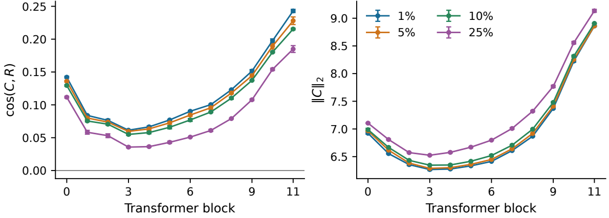
Figure 7: Archived per-block geometry. Left: contamination–recovery cosine. Right: contamination displacement norm. Error bars are sample SD across three seeds. Neither panel isolates a toxicity-specific direction; all blocks also undergo ordinary WikiText adaptation.
