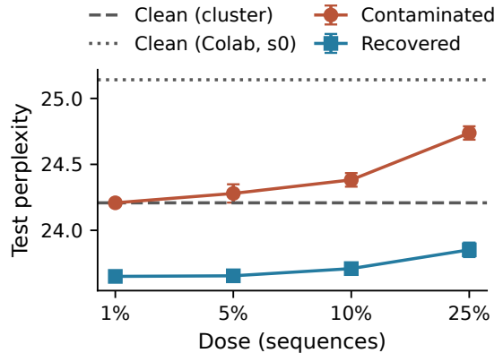
Figure 6: WikiText-103 test perplexity of the final checkpoints. Error bars are sample SD across three seeds. Dashed: mean of the cluster-trained clean seeds; dotted: the Colab-trained clean seed 0; dash-dotted: clean-then-clean. Pretrained GPT-2 scores 51.19.
