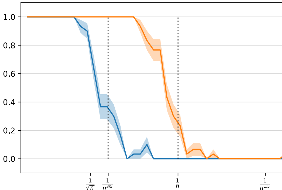
Probability of a (broken) cycle in \Gamma(n, p) as a function of p(n)
