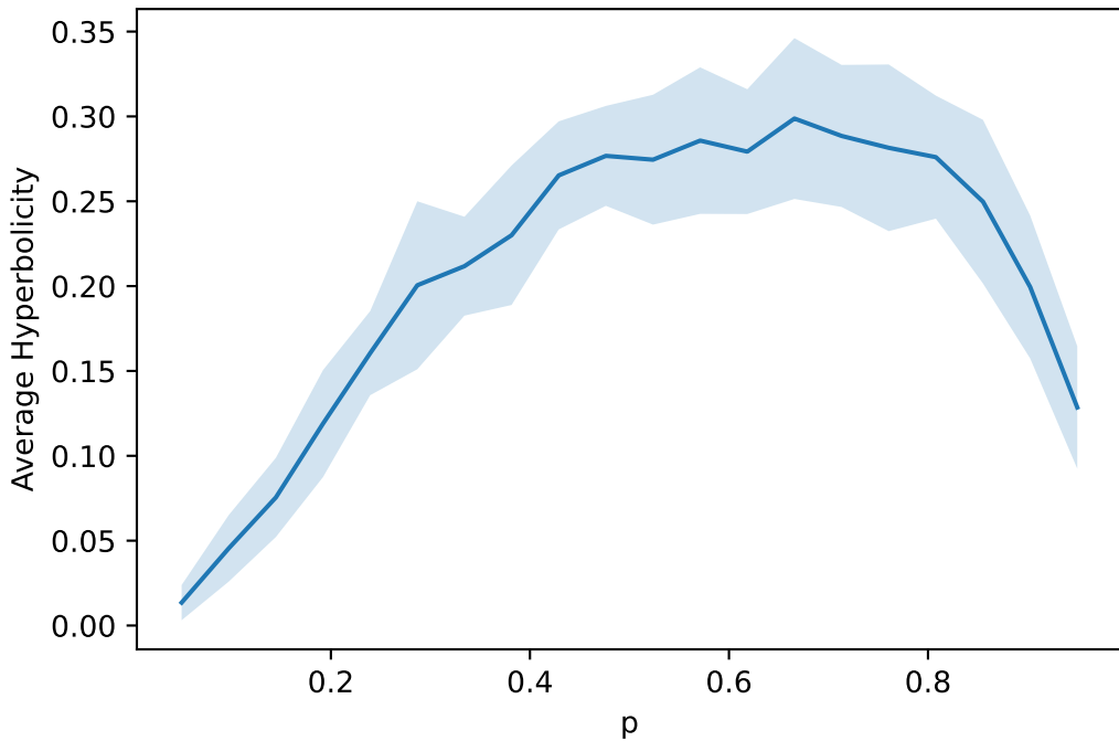
Average Hyperbolicity of G(n, p) , n = 3000
