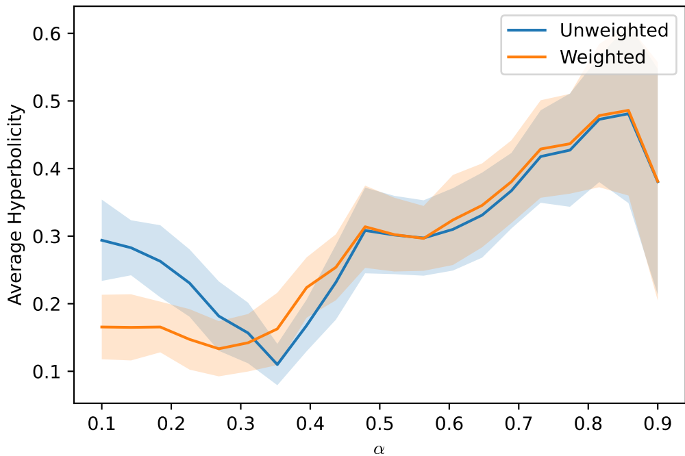
Average Hyperbolicity vs \alpha ( n = 130 , 30 reps, 30 fp conditions)
