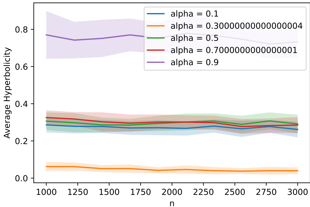
Average Hyperbolicity vs n, multiple \alpha
