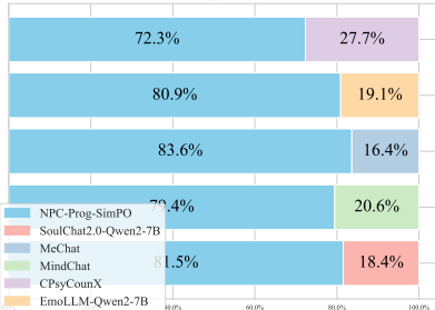
Human
