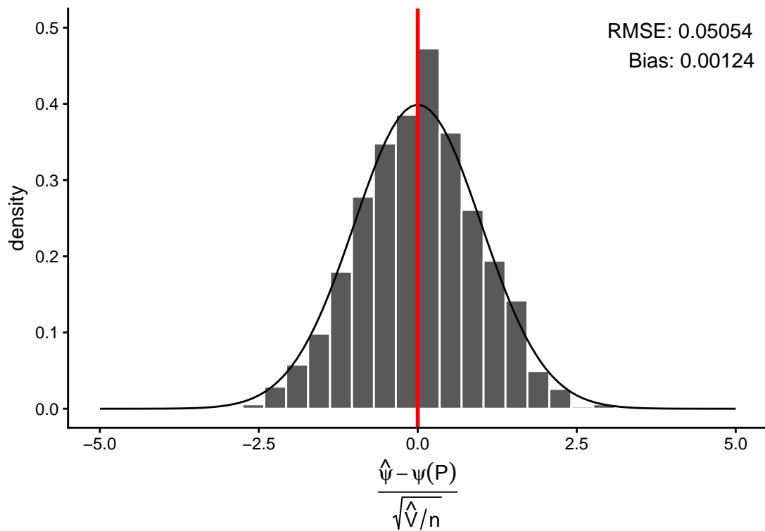
Indirect Riesz representer & Cross-fitting
