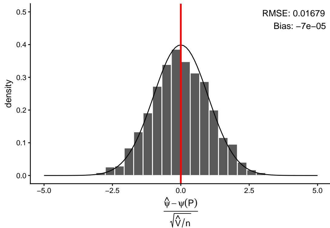
Direct Riesz representer & Cross-fitting
