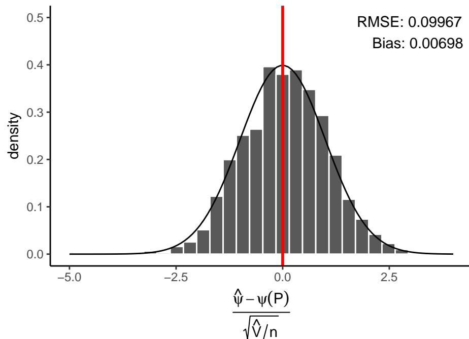
Direct Riesz representer & Cross-fitting
