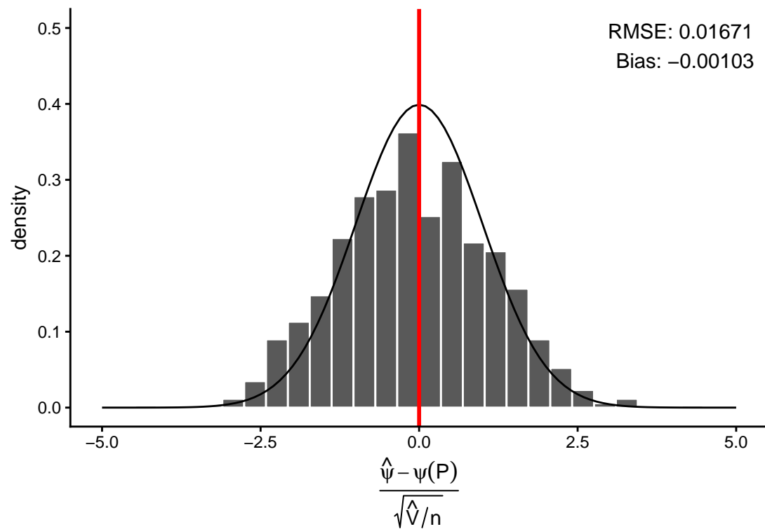
Direct Riesz representer & No cross-fitting
