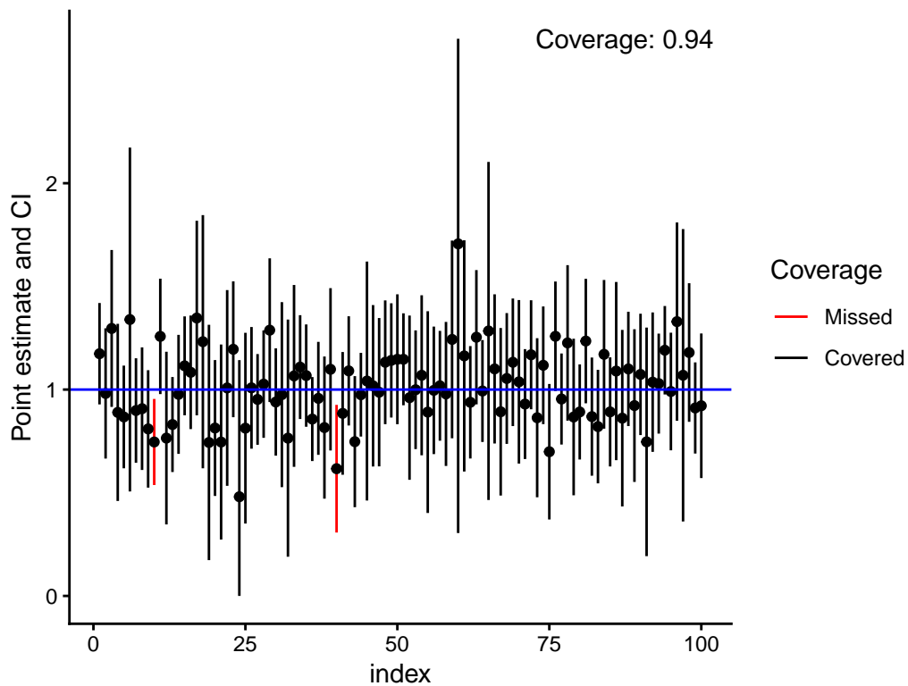
Indirect Riesz representer & Cross-fitting
