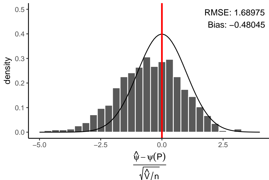
Indirect Riesz representer & Cross-fitting
