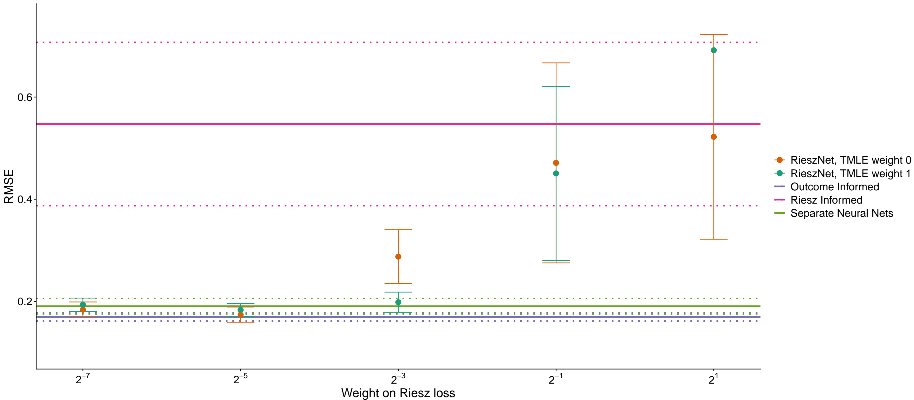
RMSE for varying weights on Riesz loss
