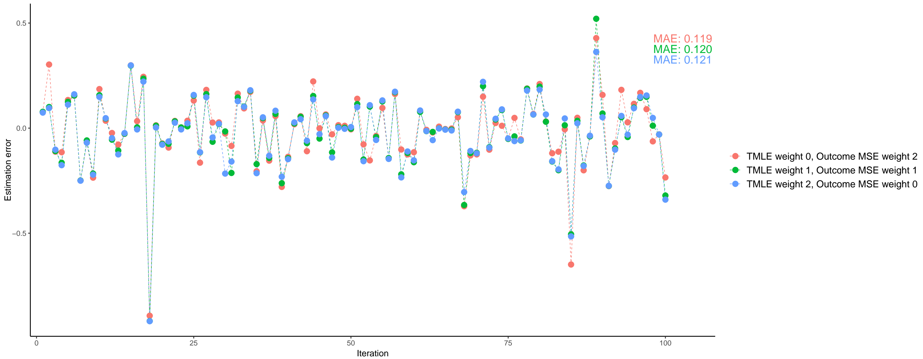
RieszNet estimation error in first 100 iterations
