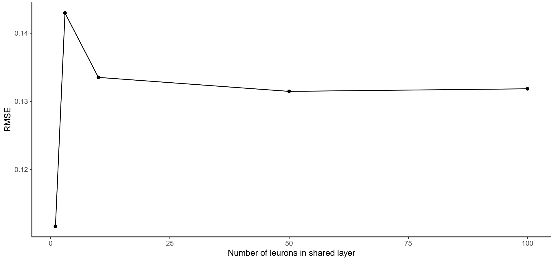
RMSE With Varying Number of Neurons in Shared Layer
