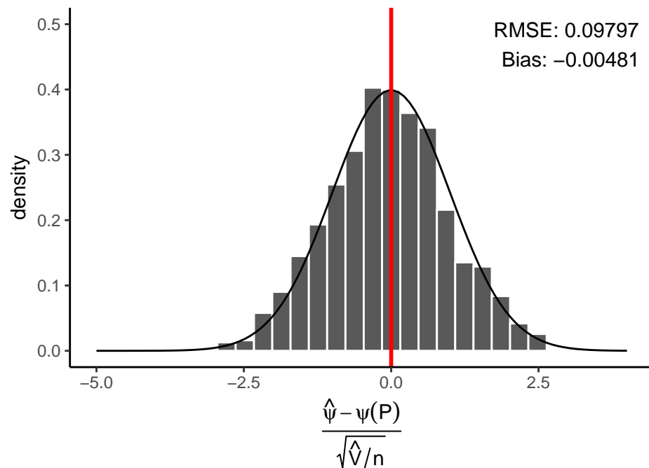
Indirect Riesz representer & Cross-fitting
