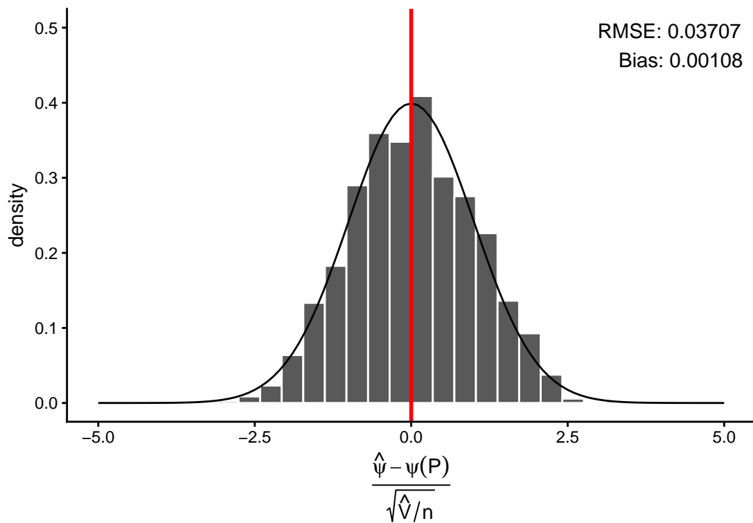
Indirect Riesz representer & No cross-fitting
