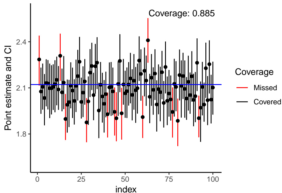
Direct Riesz representer & Cross-fitting
