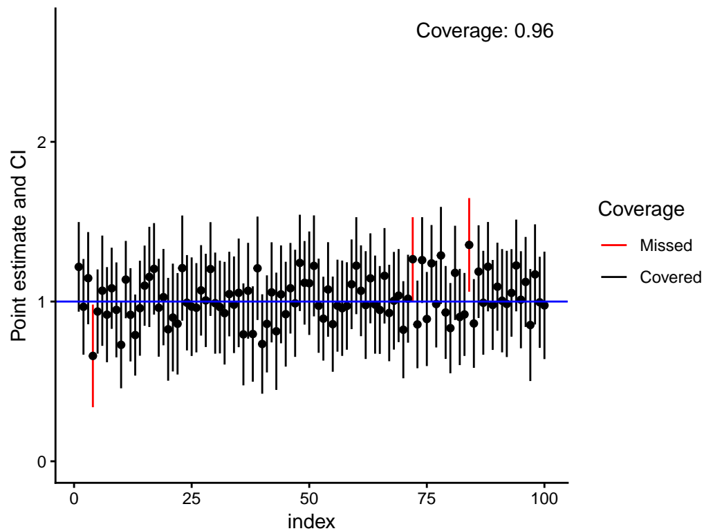
Direct Riesz representer & Cross-fitting
