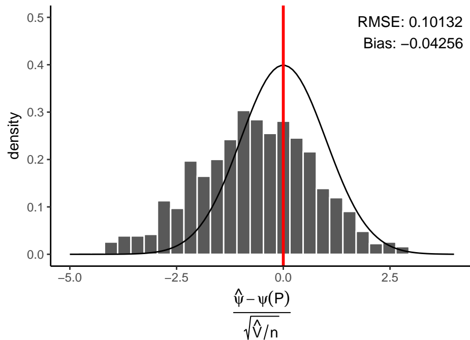
Indirect Riesz representer & No cross-fitting
