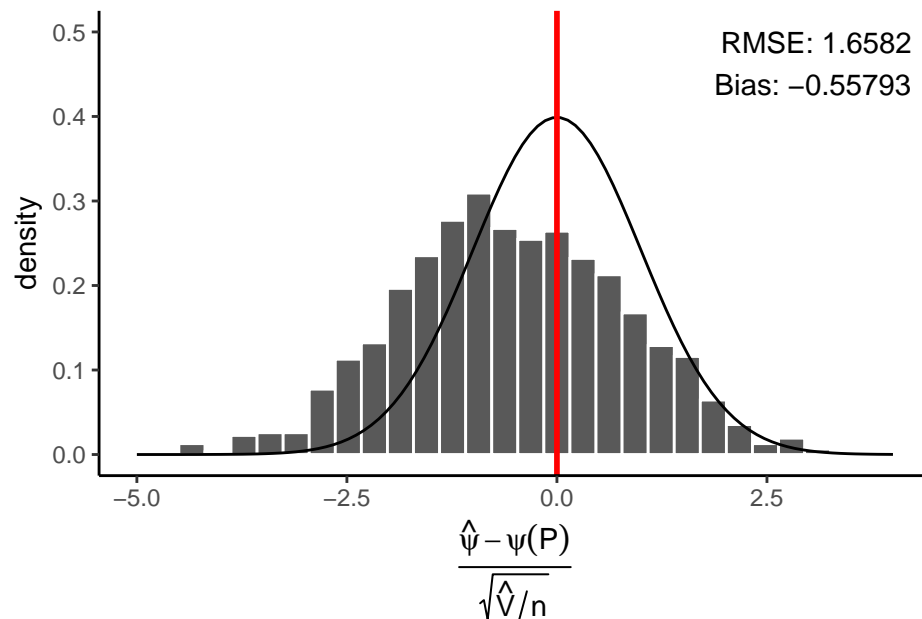
Direct Riesz representer & Cross-fitting
