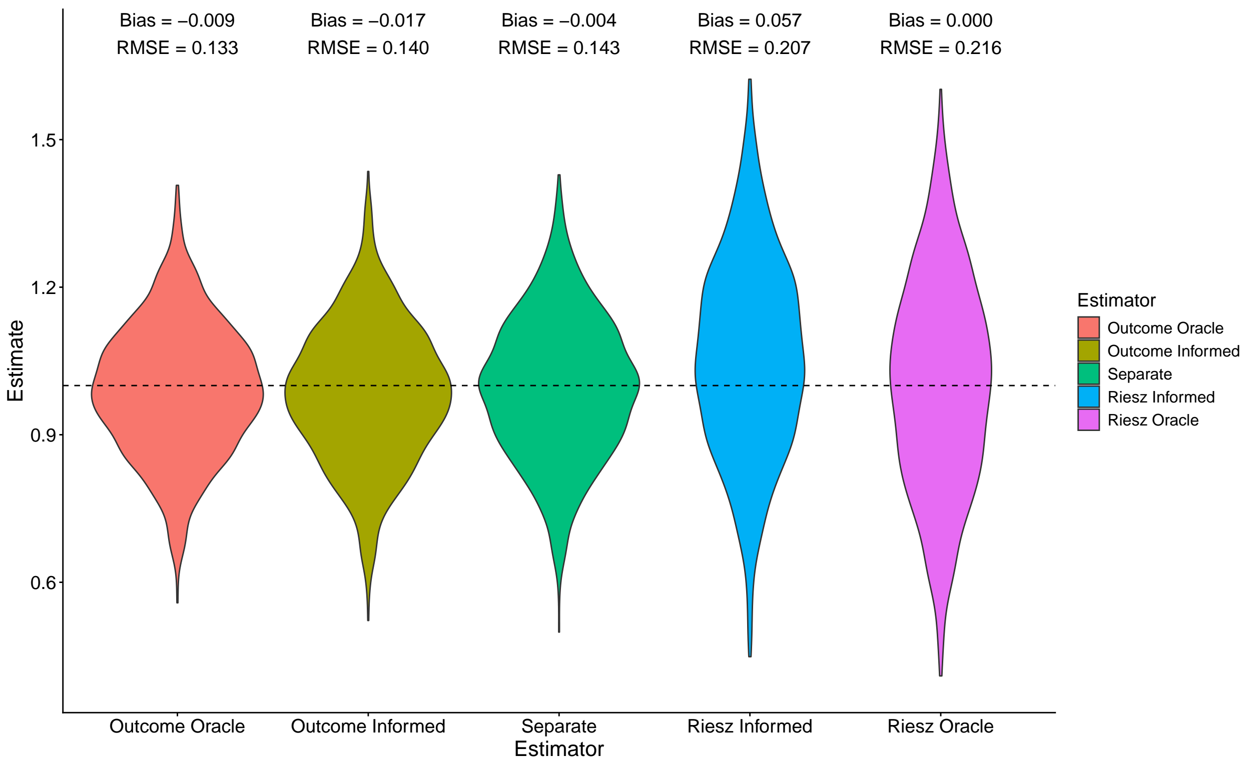
Distribution of estimators for different methods
