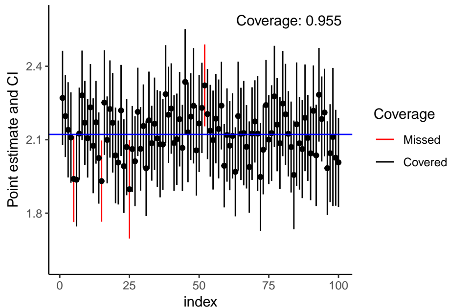
Indirect Riesz representer & Cross-fitting
