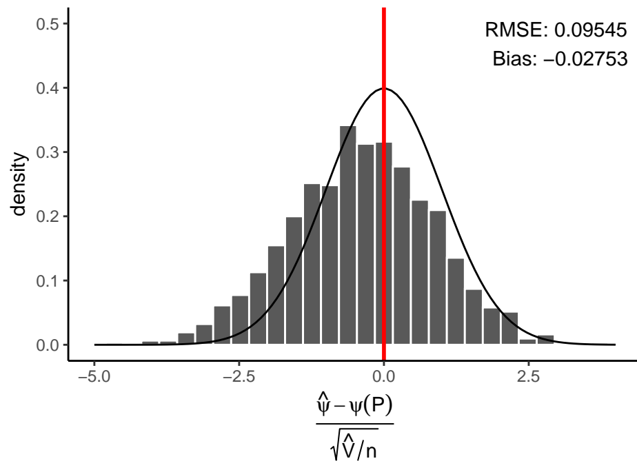
Direct Riesz representer & No cross-fitting
