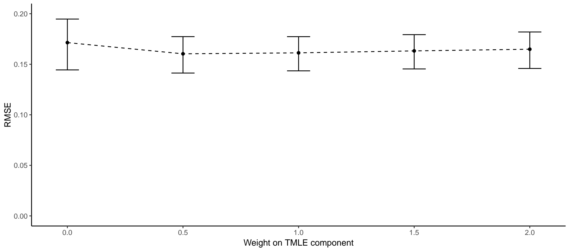
RMSE with constant total weight on TMLE and MSE loss components
