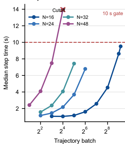
b 10-cycle runtime frontier
