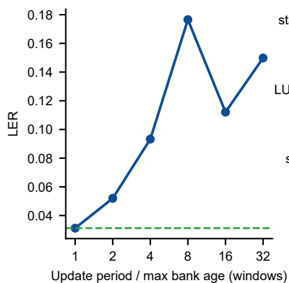
c Stale state dominates
