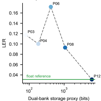
b Joint precision is not monotonic
