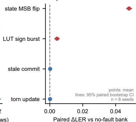
d Only severe word faults are decisive
