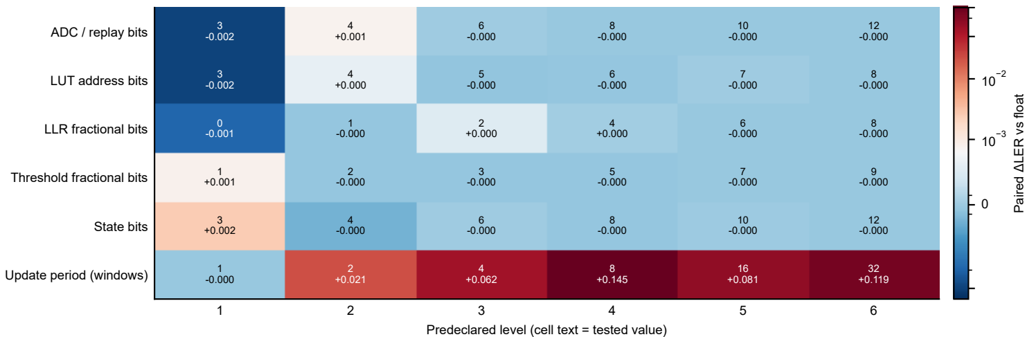
a Component precision has non-monotonic, unequal LER effects
