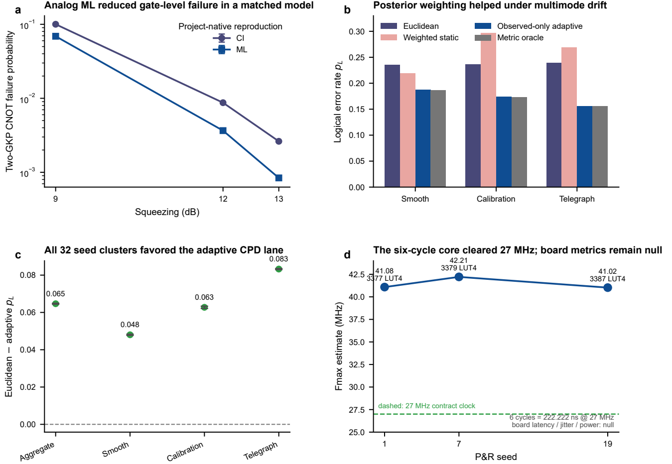
Figure 7: Bounded positive evidence outside the stopped V5 route. (a) Matched two-GKP-CNOT CI/ML reproduction; points show binomial estimates and 95% intervals. (b) Scenario LERs for the independent multimode CPD task. (c) Static-Euclidean-minus-adaptive LER is positive in the aggregate and each family; error bars are paired seed-cluster 95% intervals. (d) A source-bound six-cycle static-MAP core clears 27 MHz in three P&R seeds, but 222.222 ns is a contract-clock estimate and board latency, jitter, and power remain null. Sources: T6.17.2, T6.18.3, and T6.19.1 machine artifacts.
