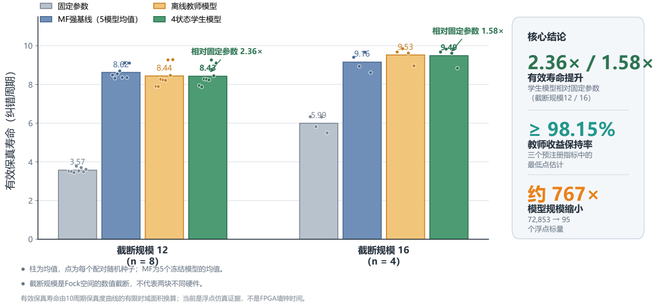
Figure 6: Finite-model teacher–student extension evidence. At cutoff 12 ( n = 8 paired evaluation seeds), the four-state student reached an effective fidelity lifetime of 8.427 cycles versus 3.571 for fixed parameters, a 2.36\times ratio. At cutoff 16 ( n = 4 ), the corresponding values were 9.489 and 5.994 cycles, a 1.58\times ratio. Bars show seed means and points show paired seeds; the MF bar is the mean of five frozen agents, not a test-selected winner. The sidebar’s 98.15% is the lowest point retention, whereas the lowest paired-bootstrap 95% interval lower bound is 94.45%. All quantities are float finite-model results.
