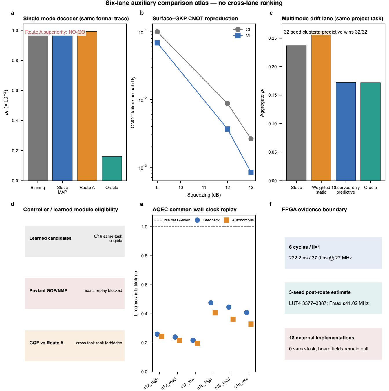
Figure 8: Integrity-gated six-lane auxiliary atlas. The panels retain, rather than hide, a single-mode Route-A NO-GO, a positive CNOT ML reproduction, a positive multimode observed-only CPD result, zero same-task learned/controller eligibility, six negative AQEC wall-clock cells, and FPGA estimate/null boundaries. The 206 cells bind report, raw source data, frozen configuration and SHA-256. The atlas has no global winner and cannot upgrade the V5 early stop or the blocked real-board gate.
