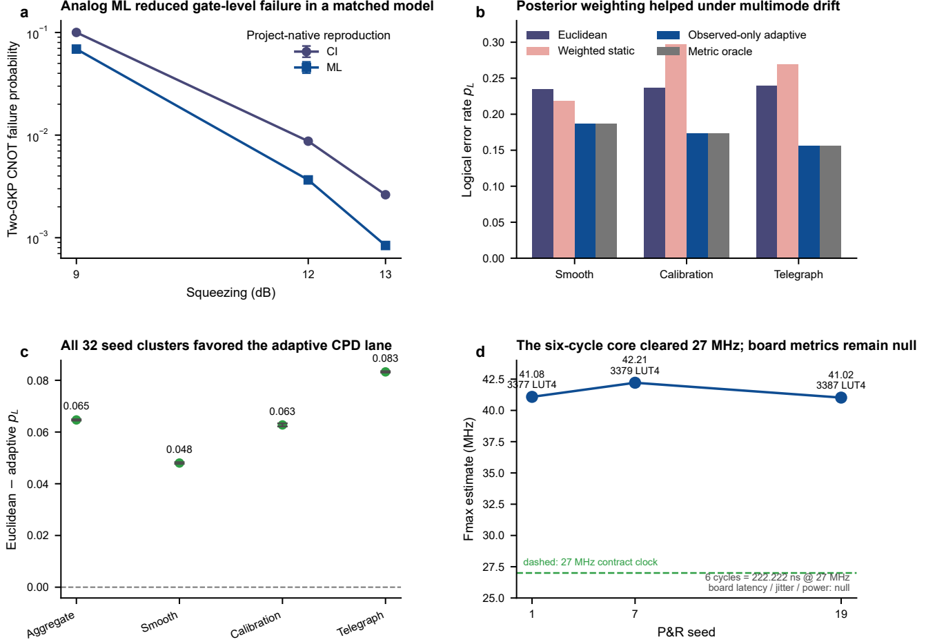
Figure 6: Bounded positive evidence outside the stopped V5 route. (a) Matched two-GKP-CNOT CI/ML reproduction; points show binomial estimates and 95% intervals. (b) Scenario LERs for the independent multimode CPD task. (c) Static-Euclidean-minus-adaptive LER is positive in the aggregate and each family; error bars are paired seed-cluster 95% intervals. (d) A source-bound six-cycle static-MAP core clears 27 MHz in three P&R seeds, but 222.222 ns is a contract-clock estimate and board latency, jitter, and power remain null. Sources: T6.17.2, T6.18.3, and T6.19.1 machine artifacts.
