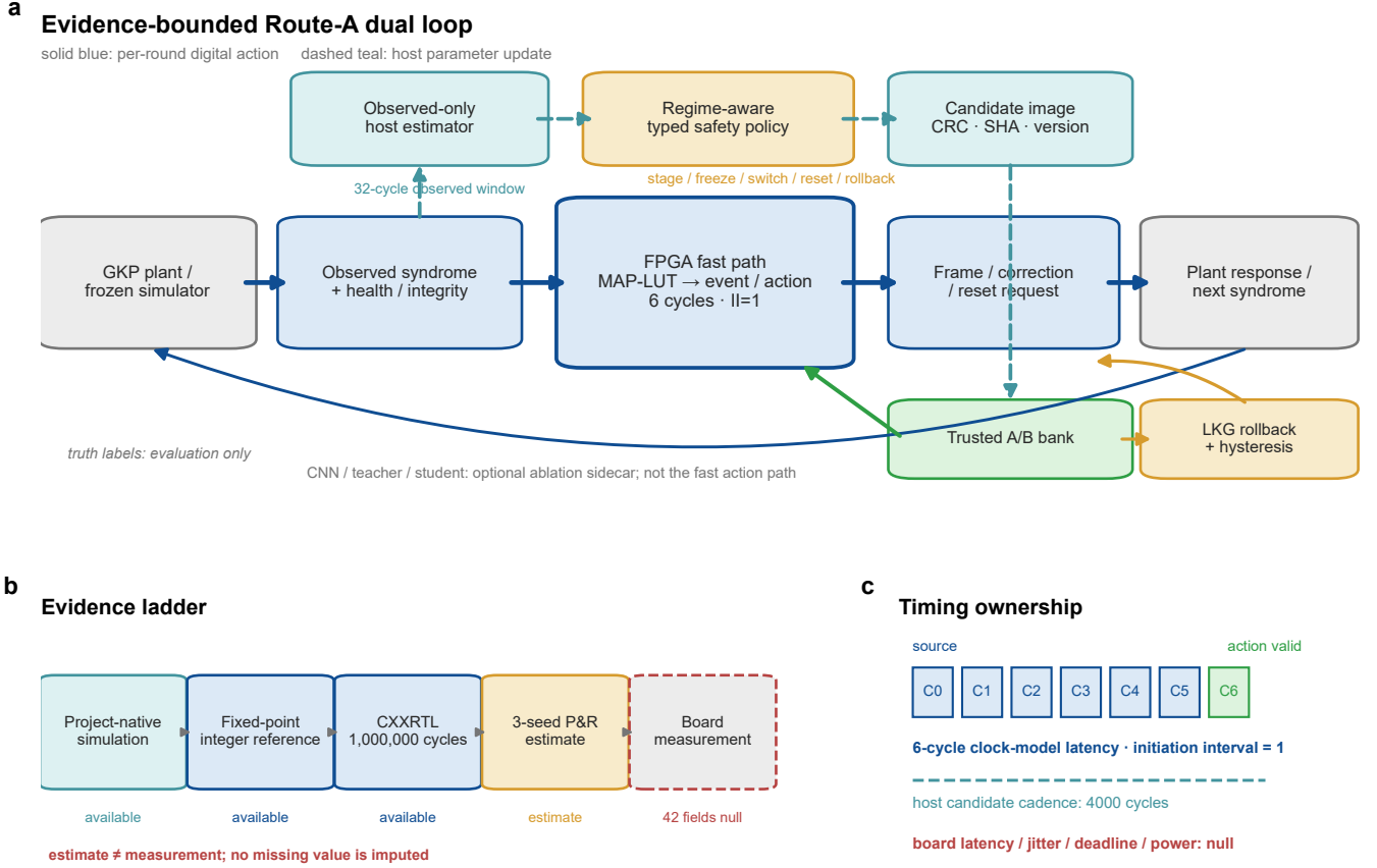
Figure 1: Current evidence-bounded ROUTE-A contract overview. The per-round MAP-LUT/event fast path is separated from the observed-only host update loop, trusted A/B publication, and LKG recovery. The evidence ladder stops at a three-seed post-route estimate; physical-board measurement remains blocked with 42 null fields. The six-cycle, II=1 timing is a pre-board clock contract, and CNN/teacher/student remain optional ablations.
