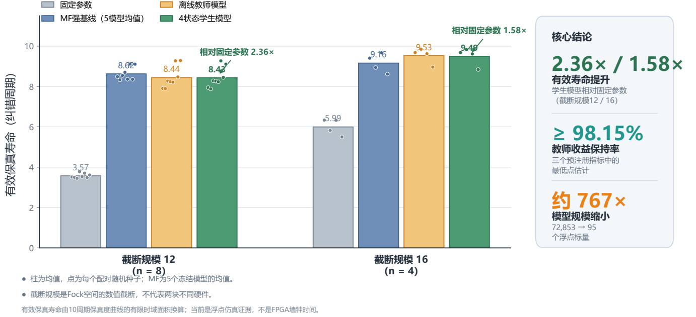
Figure 5: Reused teacher–student presentation result. The four-state student achieved 2.36× and 1.58× the fixed-parameter effective-fidelity lifetime at cutoffs 12 and 16 and used 95 scalars versus 72,853 for the teacher. This is a ten-cycle finite-model extension metric, not LER, wall-clock lifetime, official GQF reproduction, or board timing.
