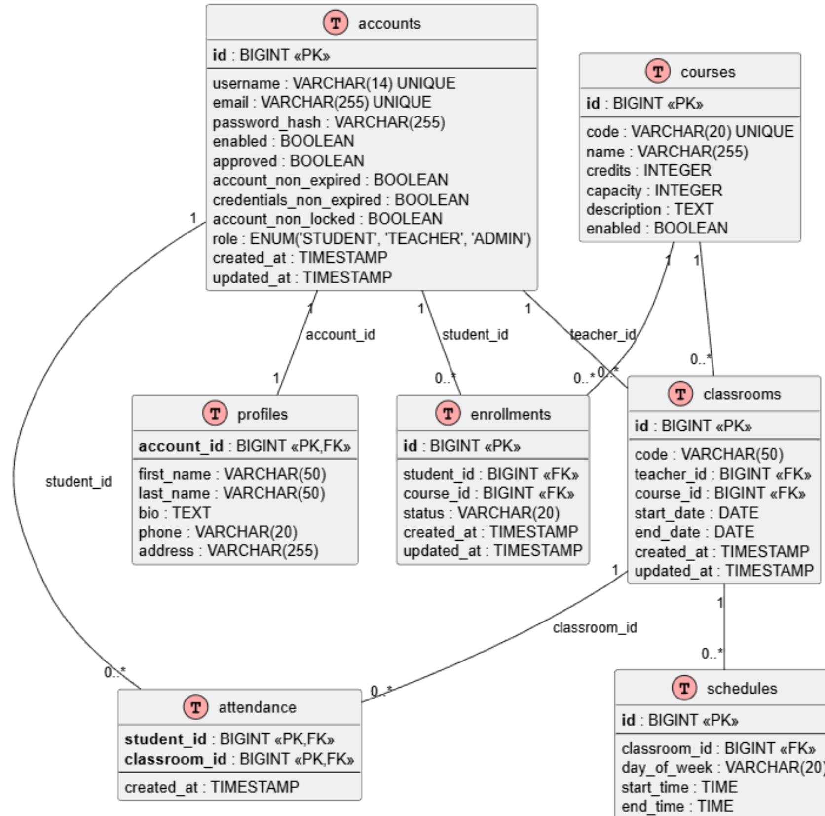
Course Enrollment System - Database Schema
