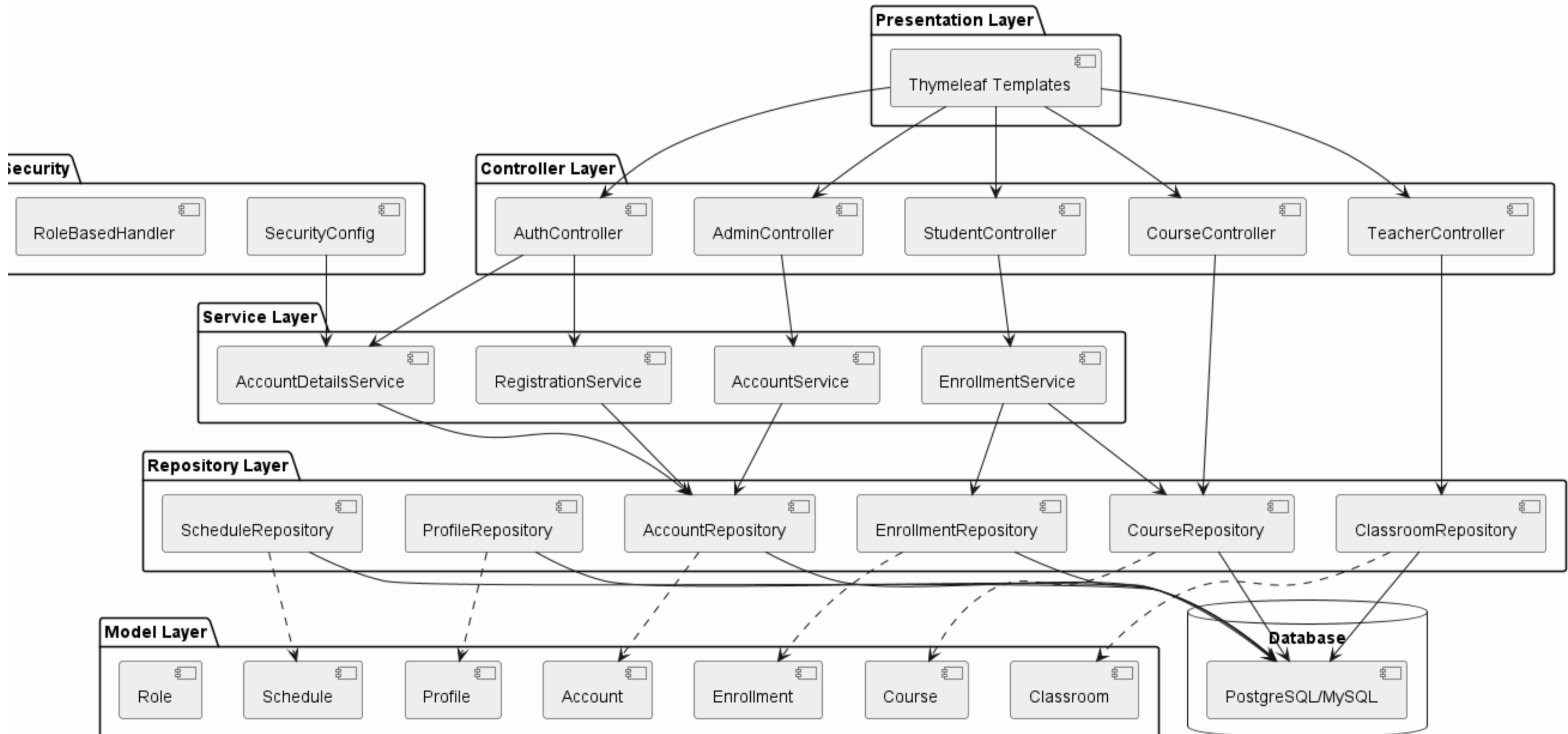
Course Enrollment System - Architecture
