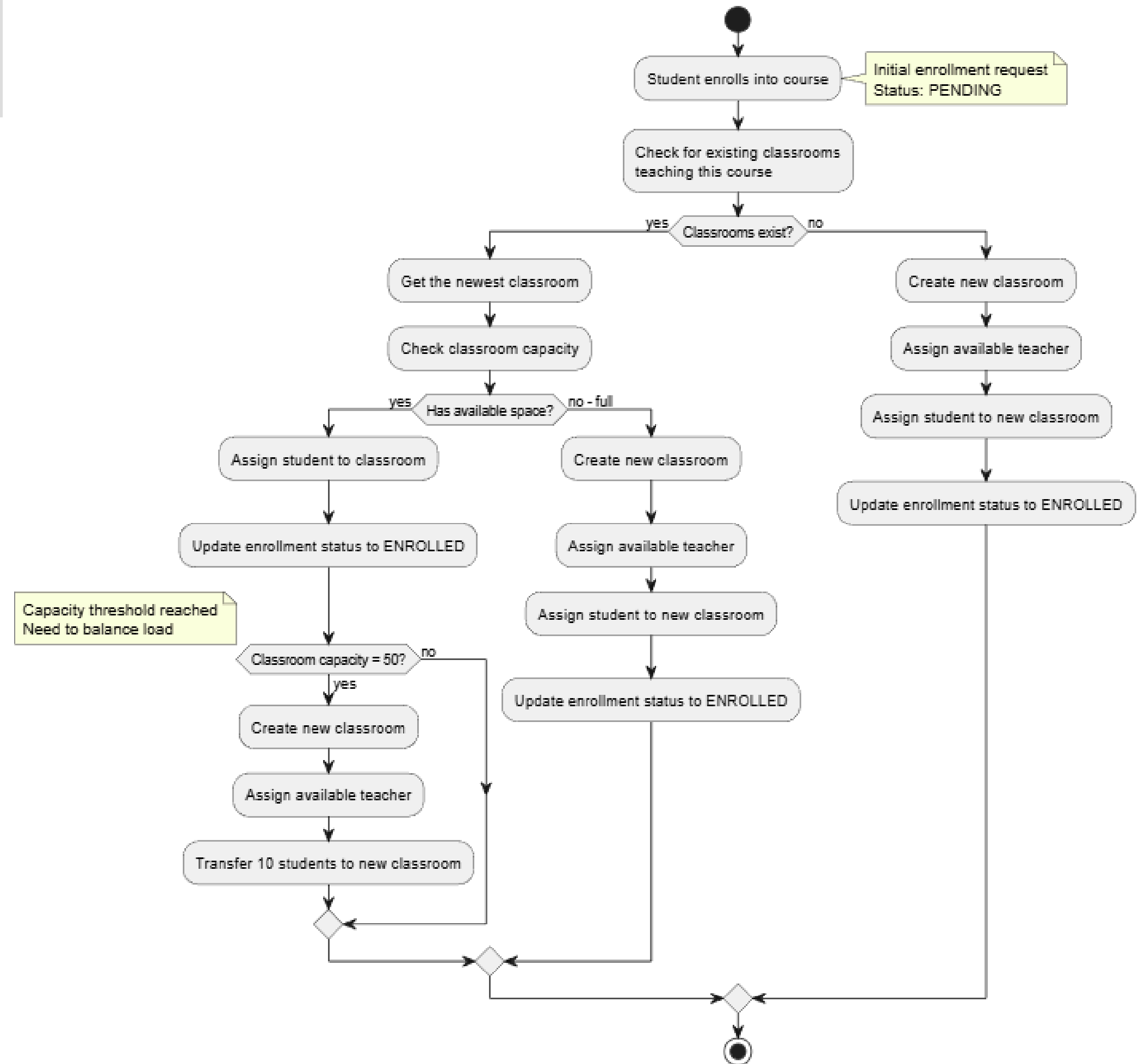
Classroom Assignment Flow
