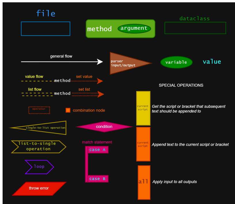
(b) Legend of the parser flowchart diagram.
