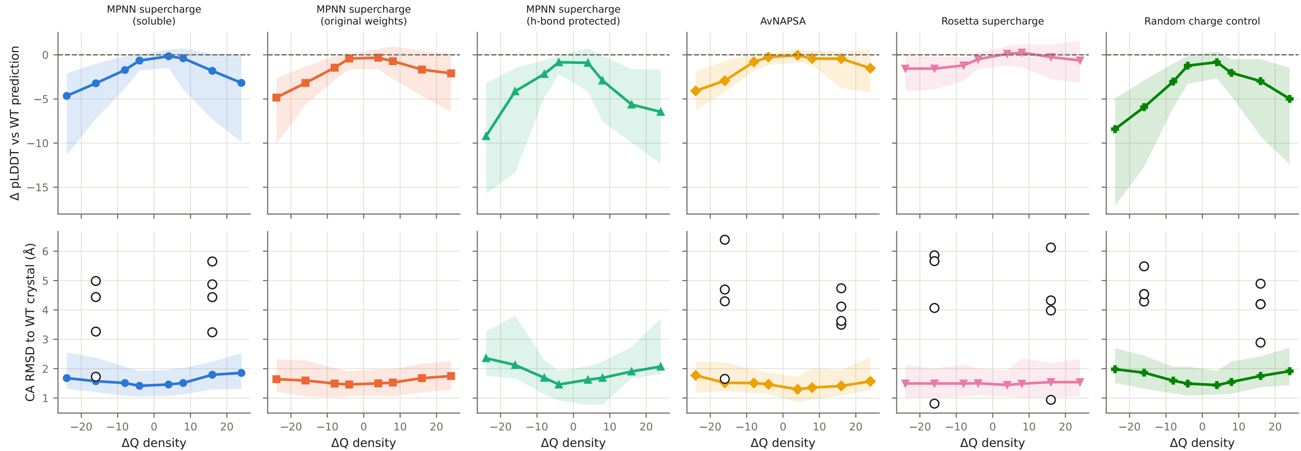
F10 Independent structure prediction. ESMFold lines with IQR ribbon; AF3 subset as open markers
