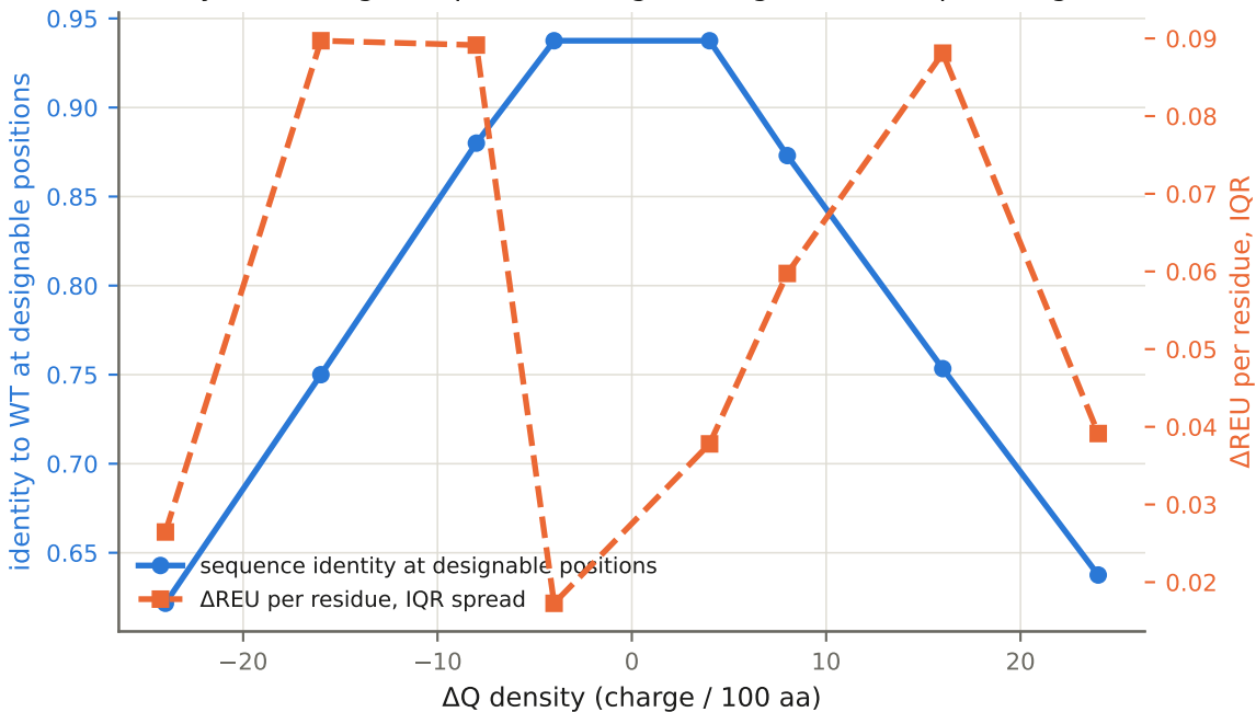
F8 Recovery and energetic spread vs target charge (MPNN supercharge (soluble))
