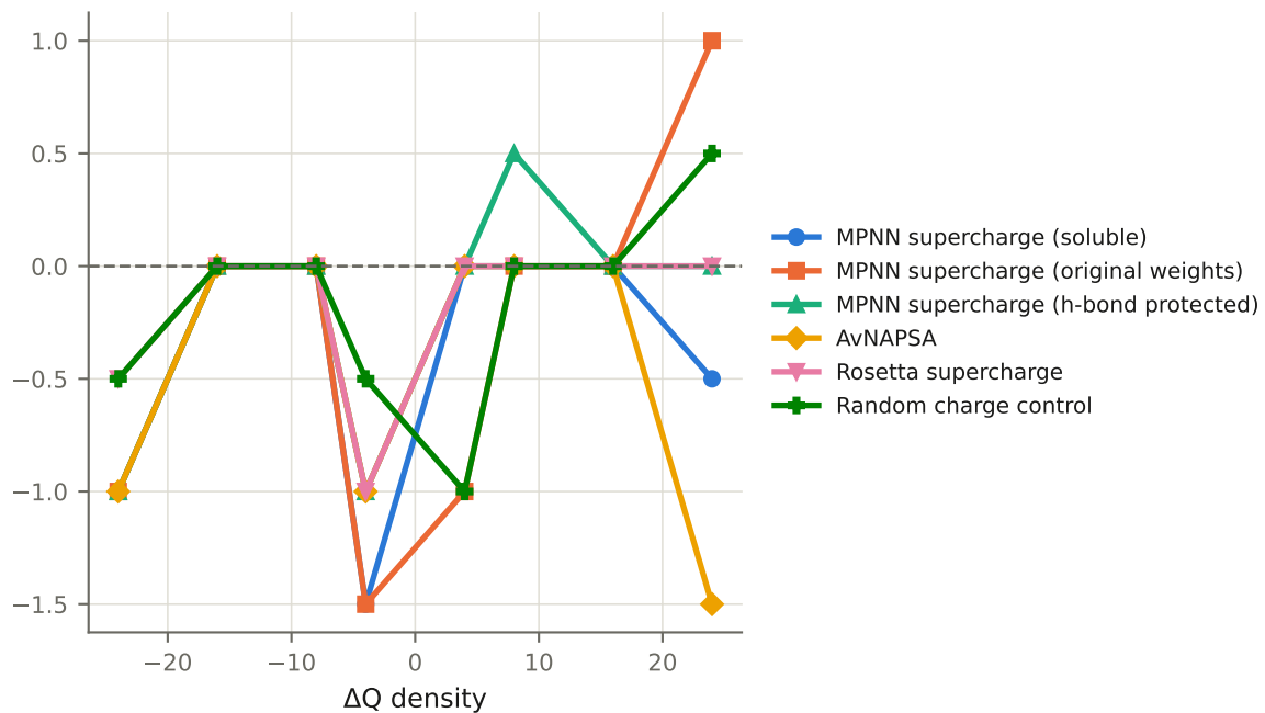
F9 \Delta side-chain H-bonds, weak ( -0.5 to -0.1 REU)
