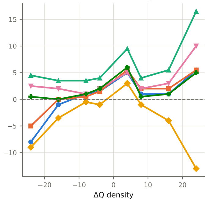
F9 \Delta side-chain H-bonds, strong ( \leq -0.5 REU)
