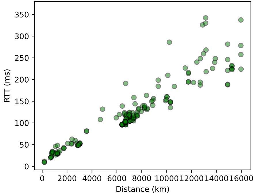
MIN RTT vs Distance
