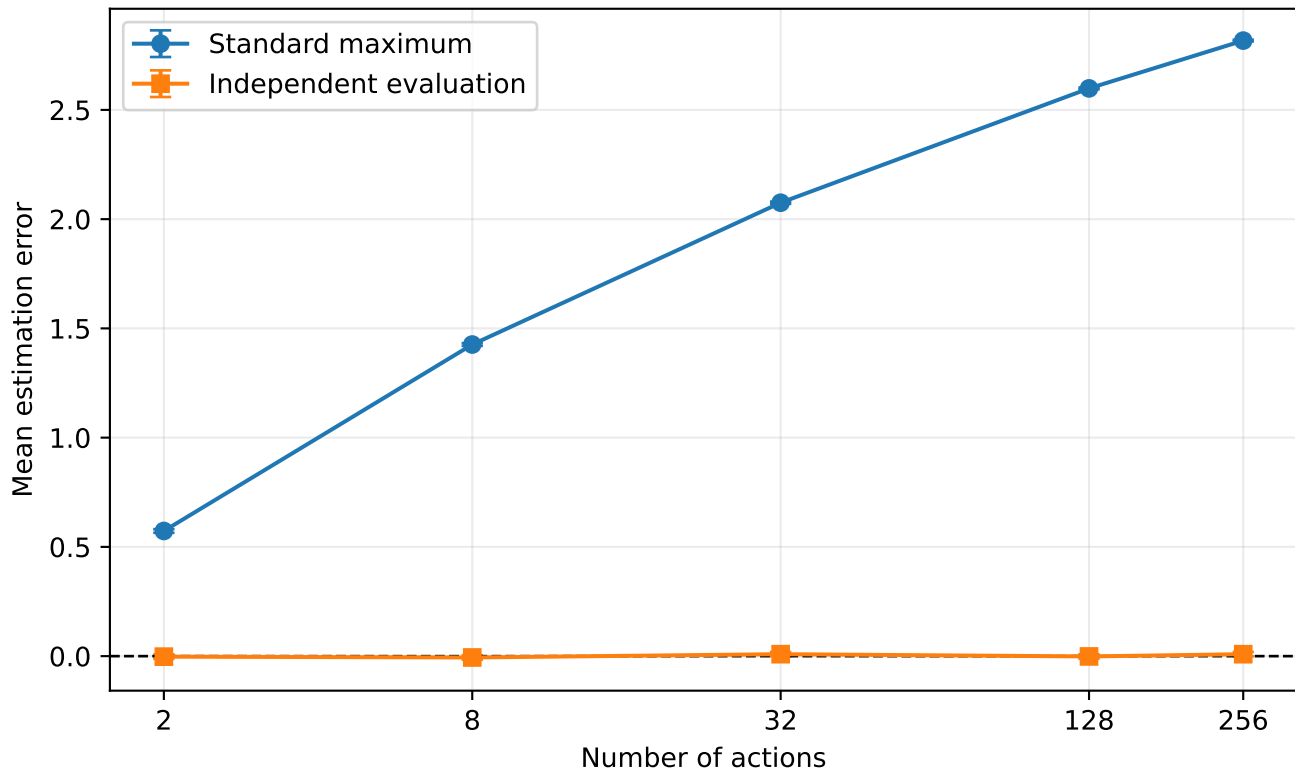
Synthetic Maximization Bias
