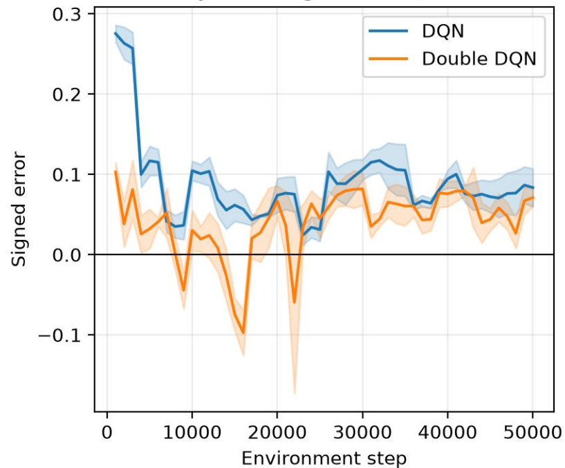
Risky-value signed error, M=10
