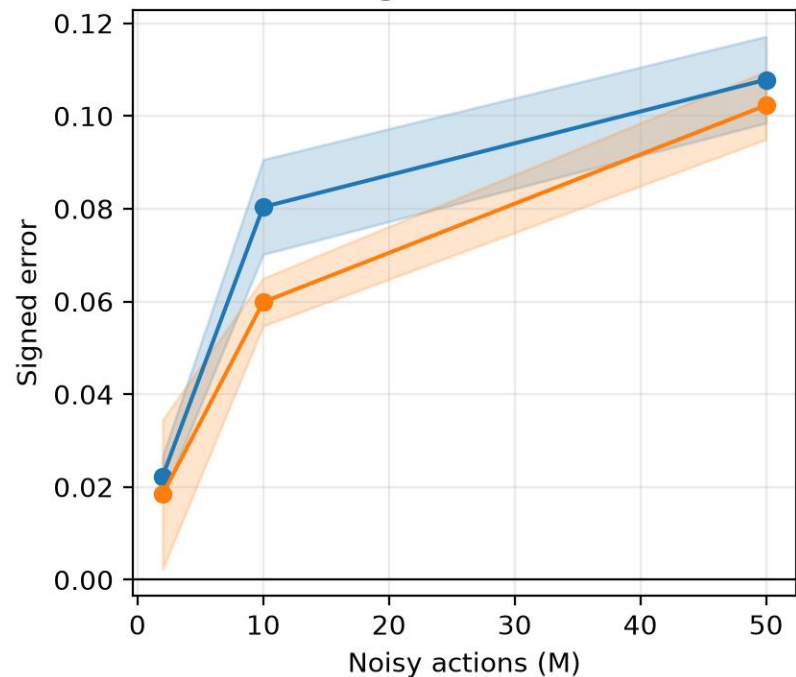
Late-training error vs action count
