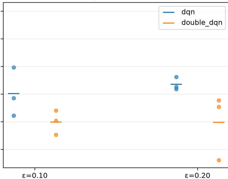
Exploration rate
