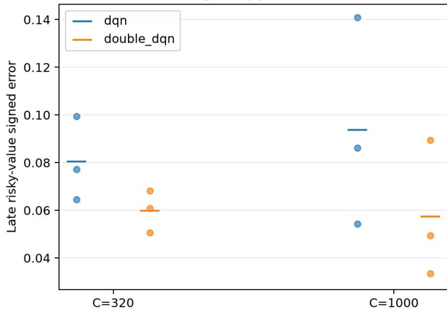
Target-copy interval
