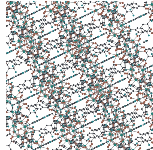
12. DB5-hypotheticalMOF_1003193_0_0_4_17_9_1
