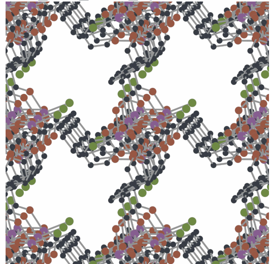
9. DB15-cds_N29_E173_opt
