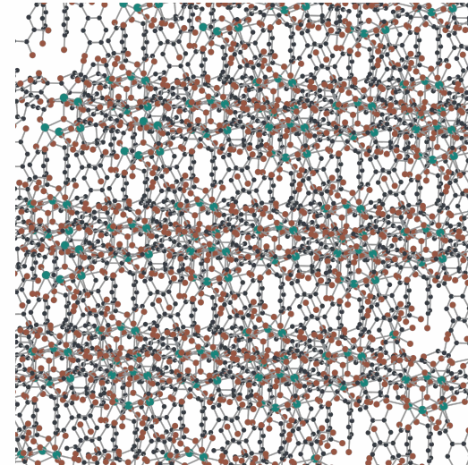
11. DB5-hypotheticalMOF_7000881_0_0_4_20_9_4
