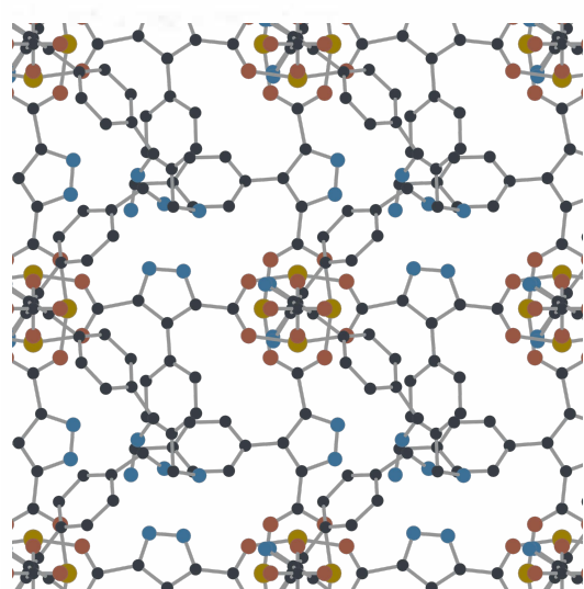
13. DB13-cds-Syn022177
