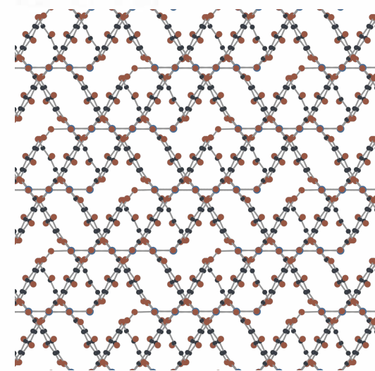
8. DB12-VAGTAA01_clean
