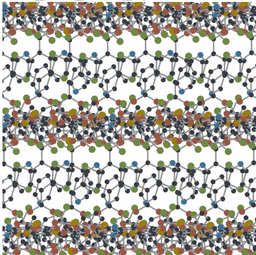
10. DB15-cds_N87_E131_opt
