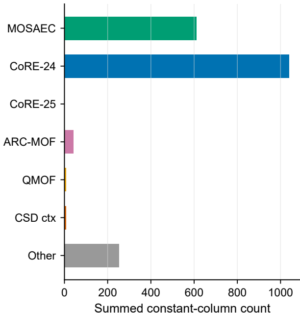
Constant columns in profiled files
