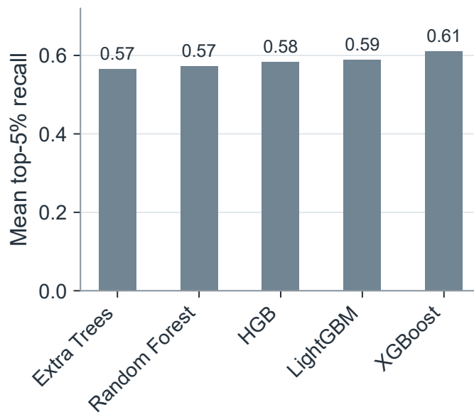
E Stable models at 1000 labels
