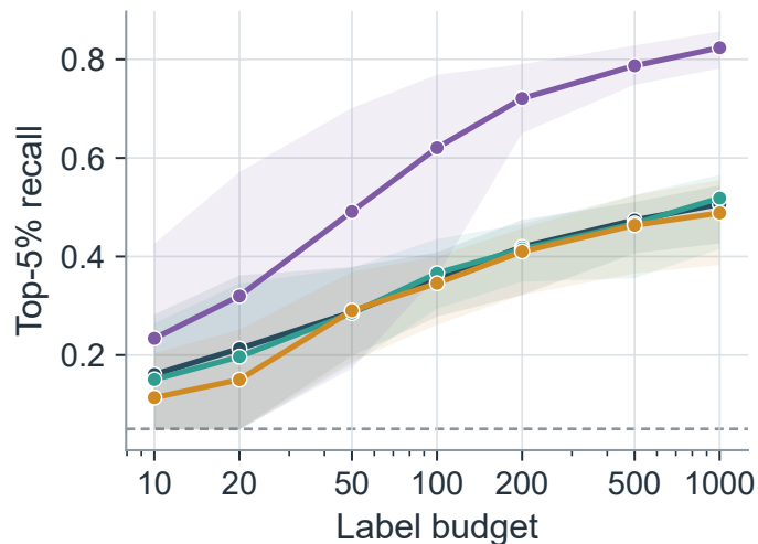
A Elite recovery from few labels
