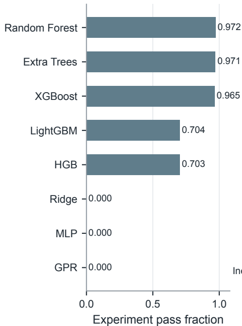
Model-family pass fraction
