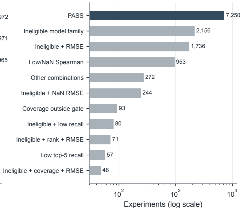
Mutually exclusive gate outcomes
