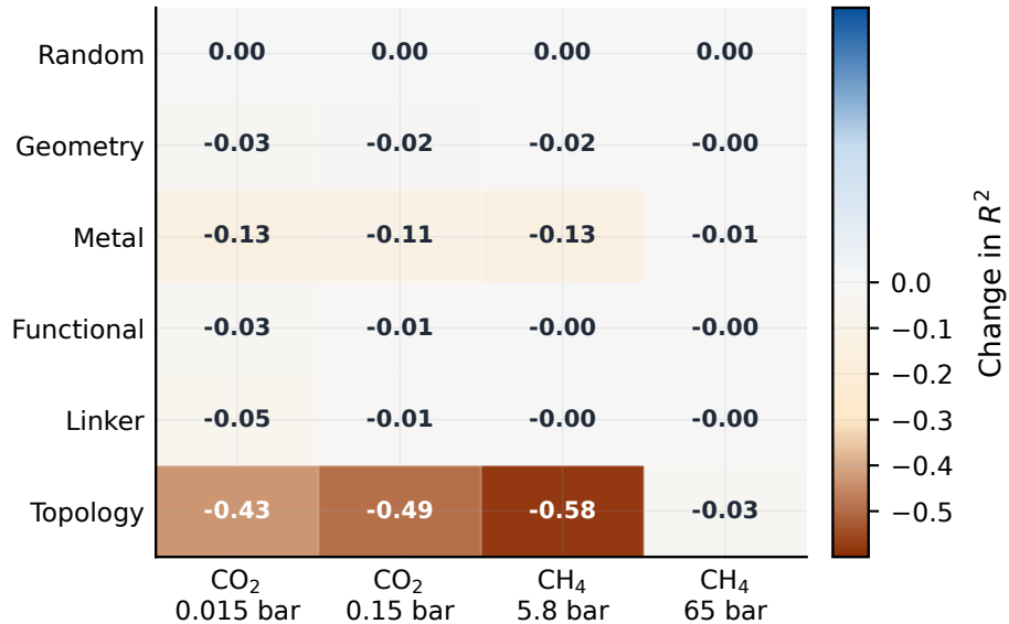
\Delta R^2 versus random split
